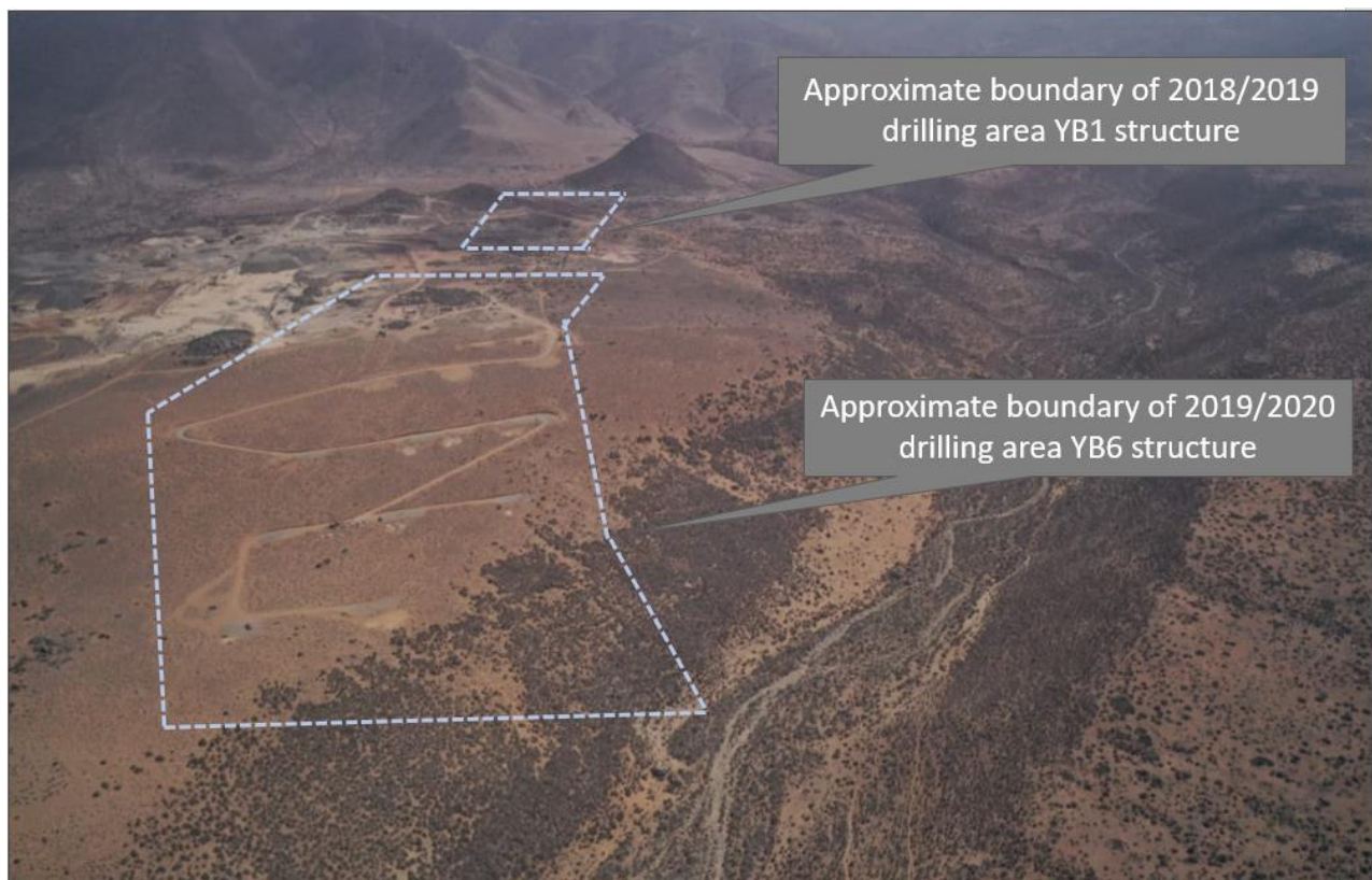
Figure 3 – Aerial photograph looking NNE showing area drilled within the YB6 magnetite project area relative to the maiden drilling program area YB1.
