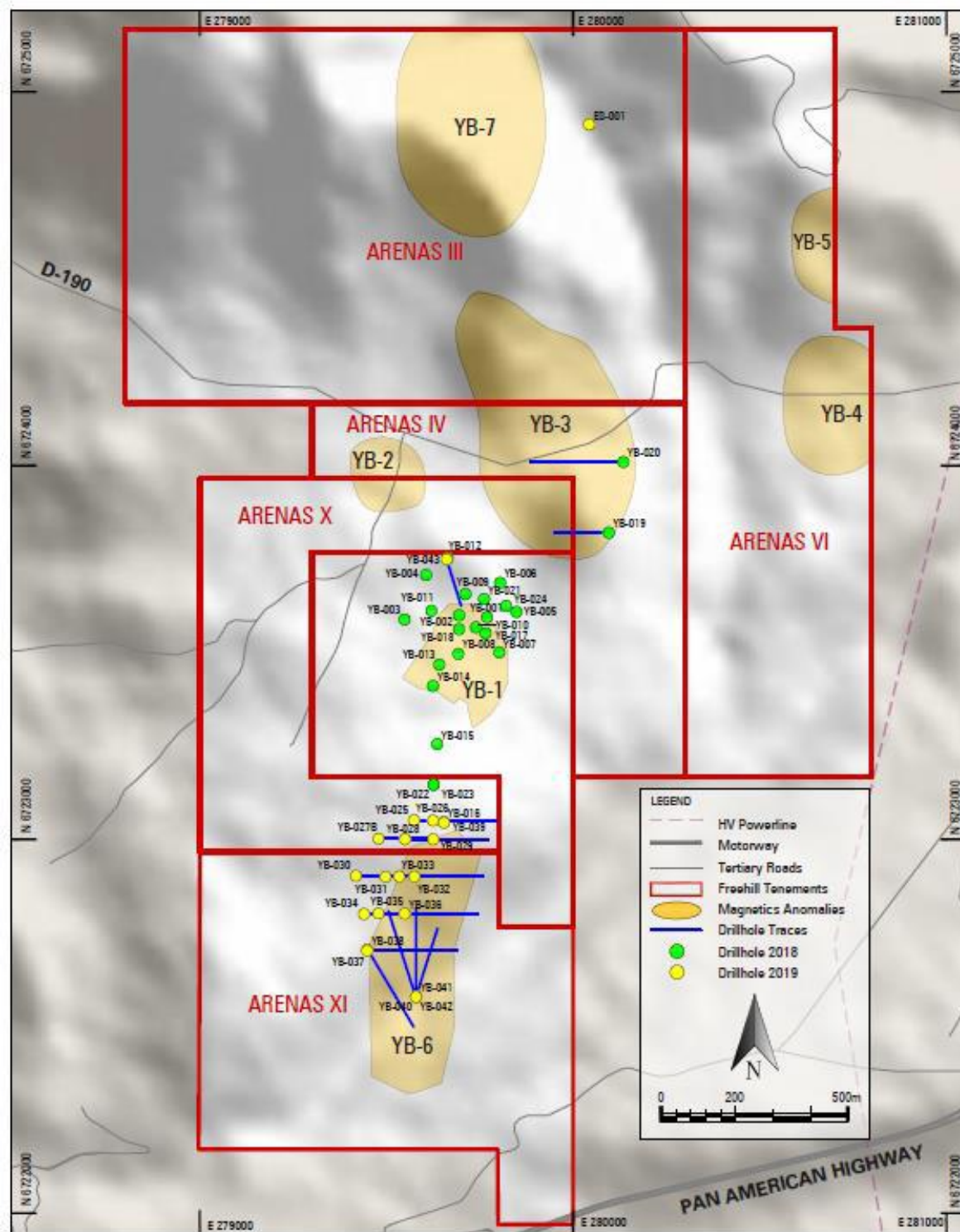
Figure 2 – Ground magnetic targets YB1-YB7 with 2018/19 (green drill holes) and 2019/20 yellow drill holes) currently defined resource areas
