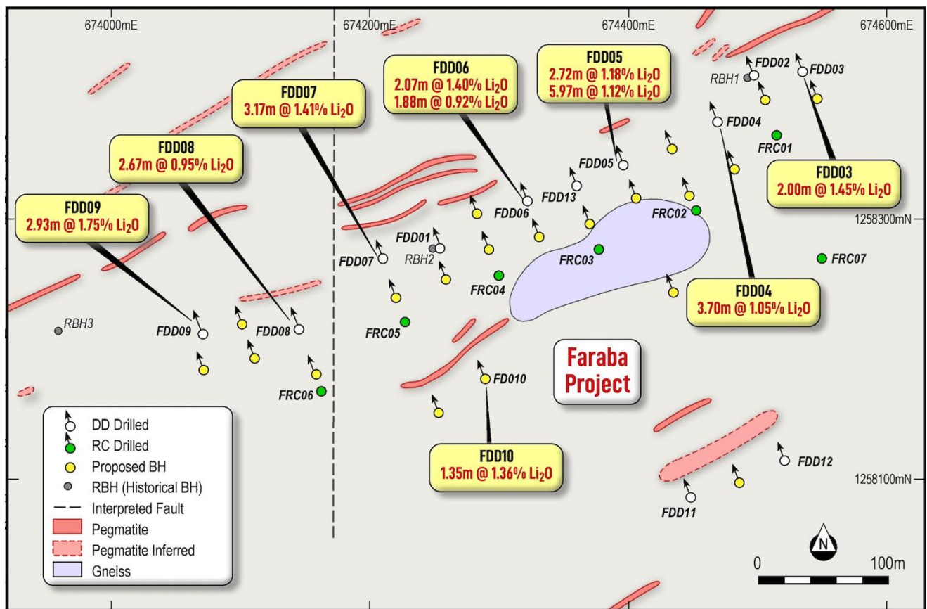
Figure 1: Locality and analytical results of Faraba diamond drill holes FDD03 to FDD010
