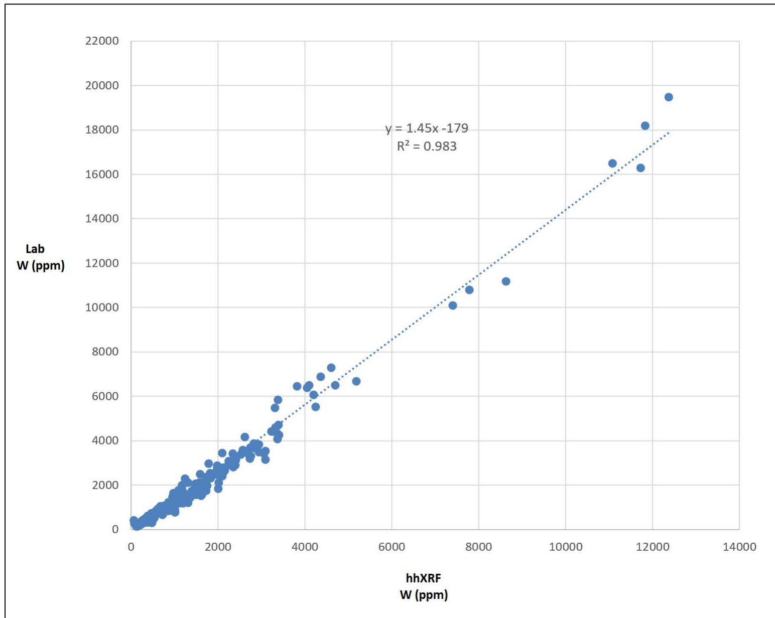
Chart A. Comparison scatterplot of laboratory derived W and hhXRF derived W from assay pulps and standards, with regression formula
