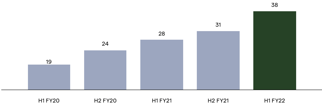
Figure 1: Contractor Customers
