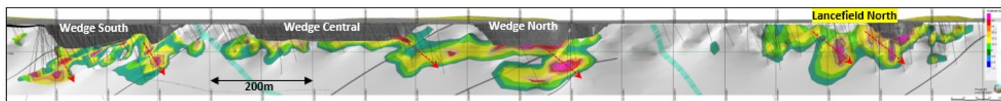
Figure 6: View West Wedge south to Lancefield North long section with contoured GxM (Grade x Width) cut-off at 5 GxM:
