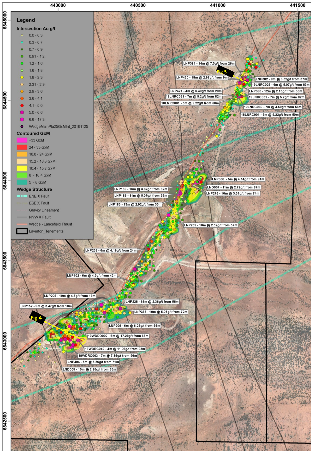
Figure 3: Wedge-Lancefield North Indicated Resource with GxM (Grade x Width) contours and drilling intersections coloured/sized by grade. Intersections exceeding 25 GxM are highlighted by labels. The locations of sections as per Figures 4 and 5 are also shown.
