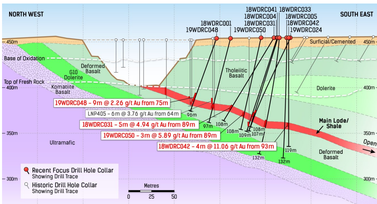
Figure 4: Wedge South cross section (looking NE) with labelled mine sequence geology, mineralised structure, historic 50m-deep Ashton Gold pit to 400mRL, drill traces with significant intersections, depth of weathering (white dashed lines). Note that due to close-spaced drilling and available space not all intersections have been labelled.
