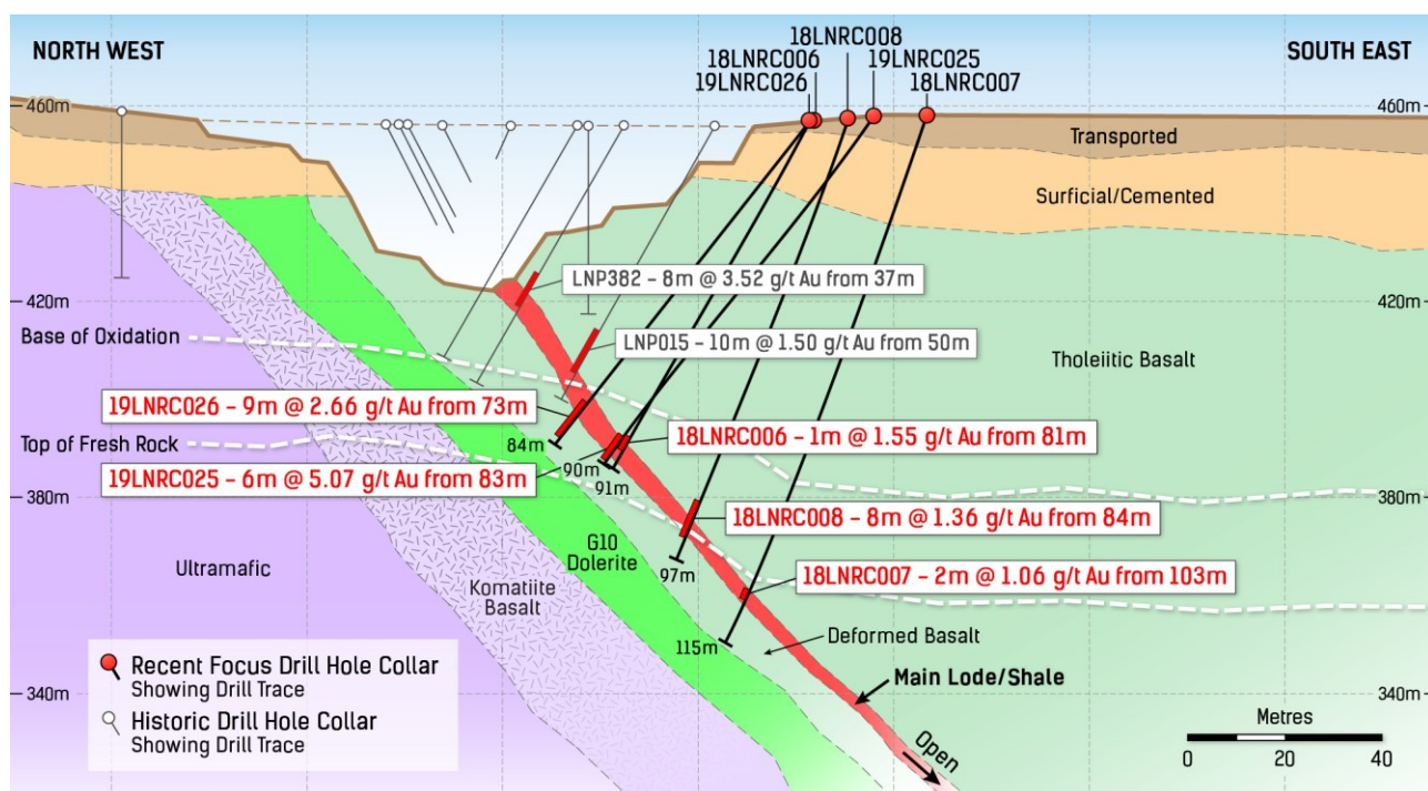
Figure 5: Lancefield North cross section (looking NE) with labelled mine sequence geology, mineralised structure, historic 30m depth Ashton Gold pit to 420mRL, drill traces with significant intersections, depth of weathering (white dashed lines).
