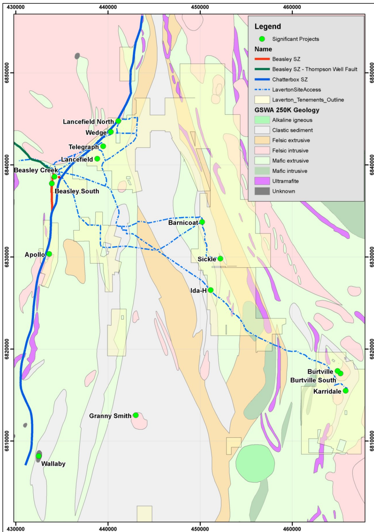
Figure 2: Regional GSWA 250K scale geology/structure map with location of Focus Minerals tenure, significant gold projects and some Laverton access roads are also shown.
