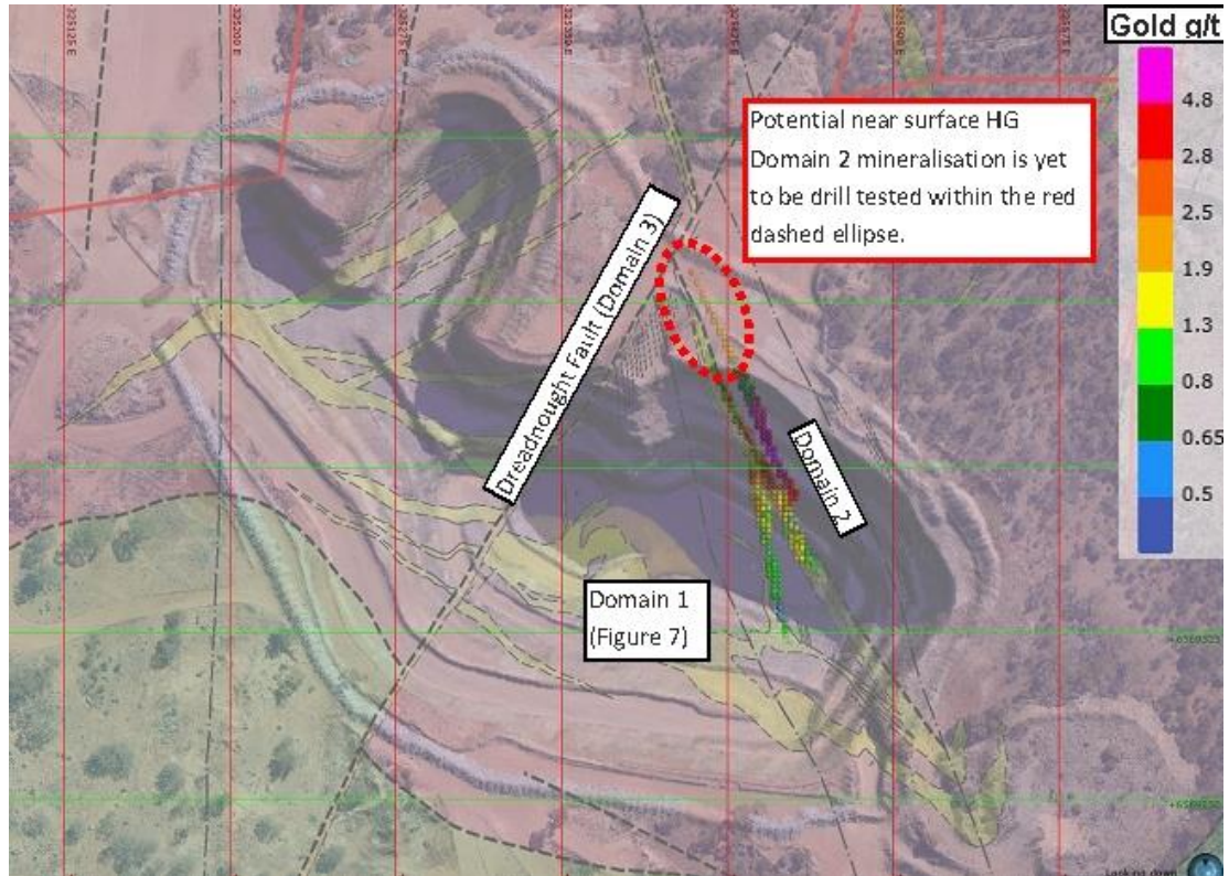
Figure 8: Plan view highlighting block model centroids for Lodes 9 to 11 within Domain 2 which dip at 84^\circ towards 250^\circ . The Block model is coloured by Au g/t as per the inset legend.
