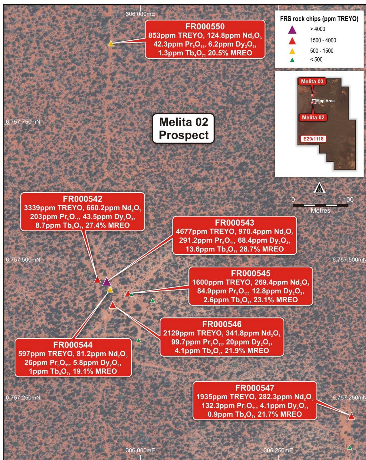
Figure 2: Strong REE geochemical results from the Melita 02 prospect, at the Breakaway Well project (E29/1118). (Samples over 590ppm TREYO are labelled with their corresponding Nd, Pr, Dy and Tb oxide results. MREO % number is the ratio of MREO to TREYO)
