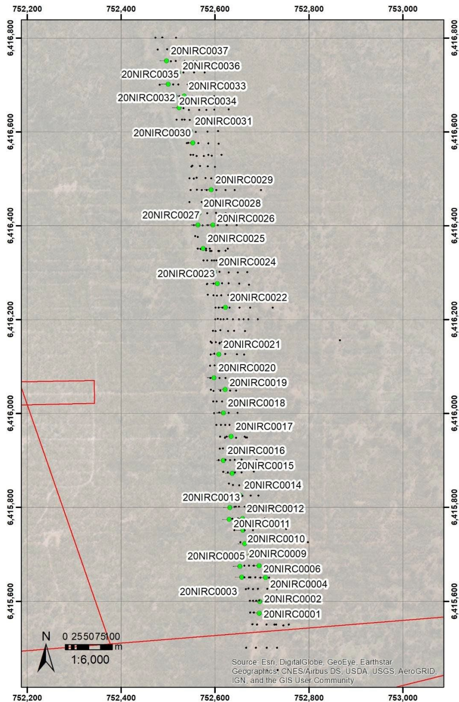
Figure 5 –Recent RC drilling operations at the North Ironcap gold project (M77/544)
