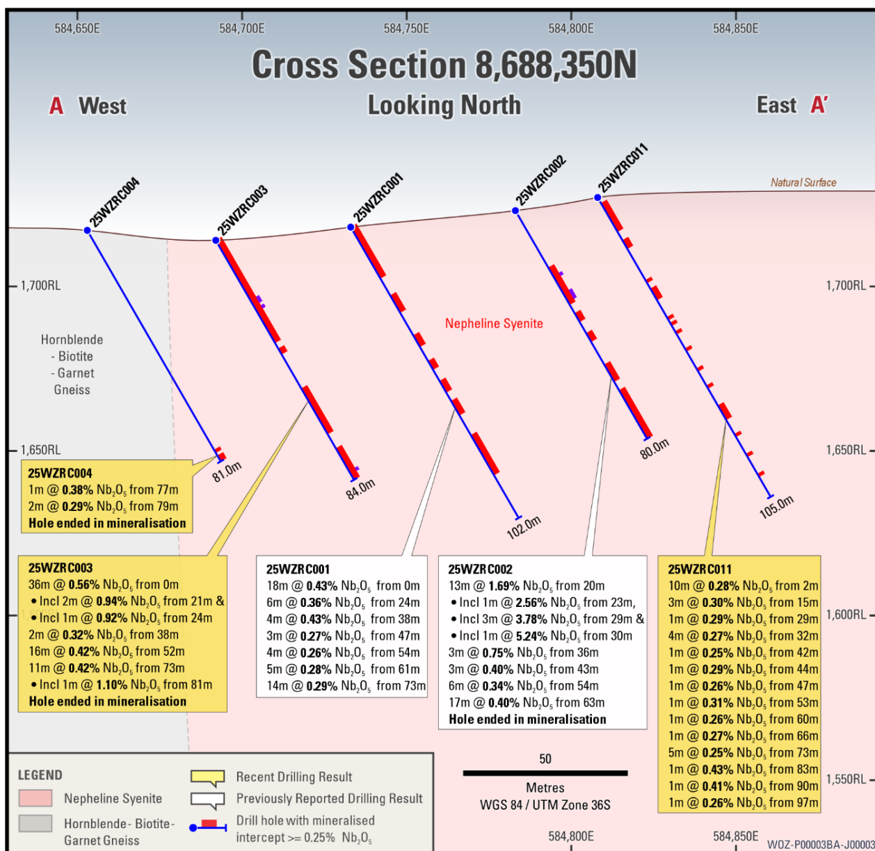
Figure 6: Cross-section 8,688,350 N
