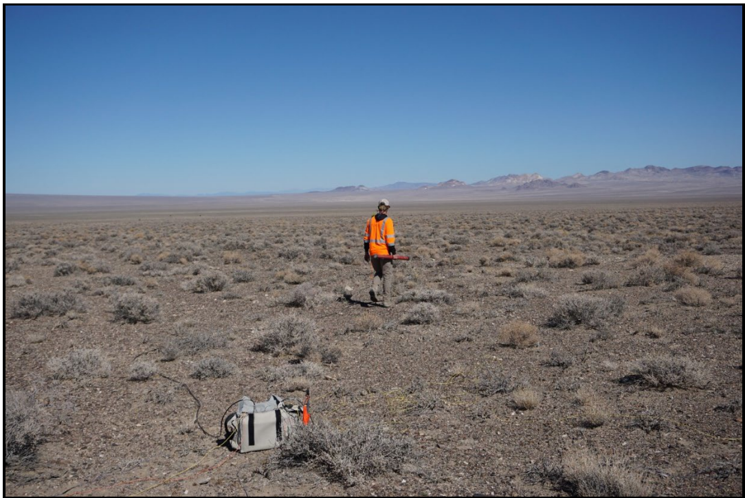
CSAMT SURVEY RECIEVER DEPLOYMENT AT THE ALKALI FLATS PROJECT
