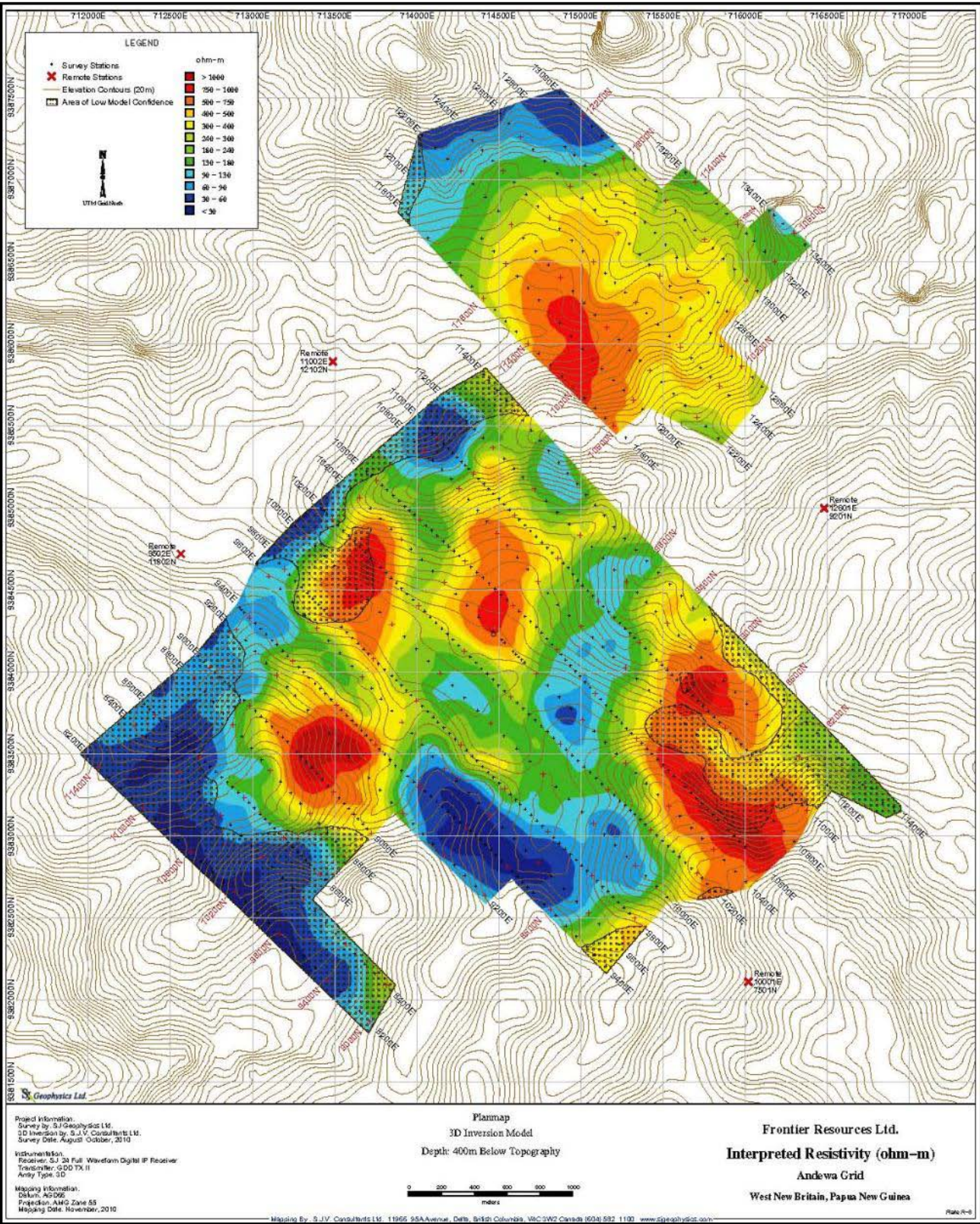
Figure 11. Interpreted resistivity at 400m depth below topography.
