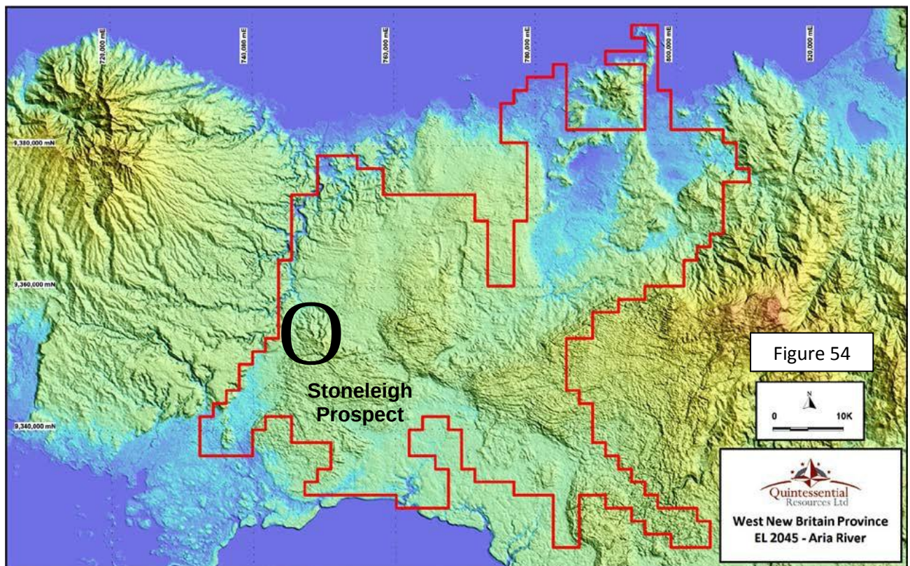
Figure 54 : SRTM topographic image showing EL 2045 Aria River and the Stoneleigh Prospect
