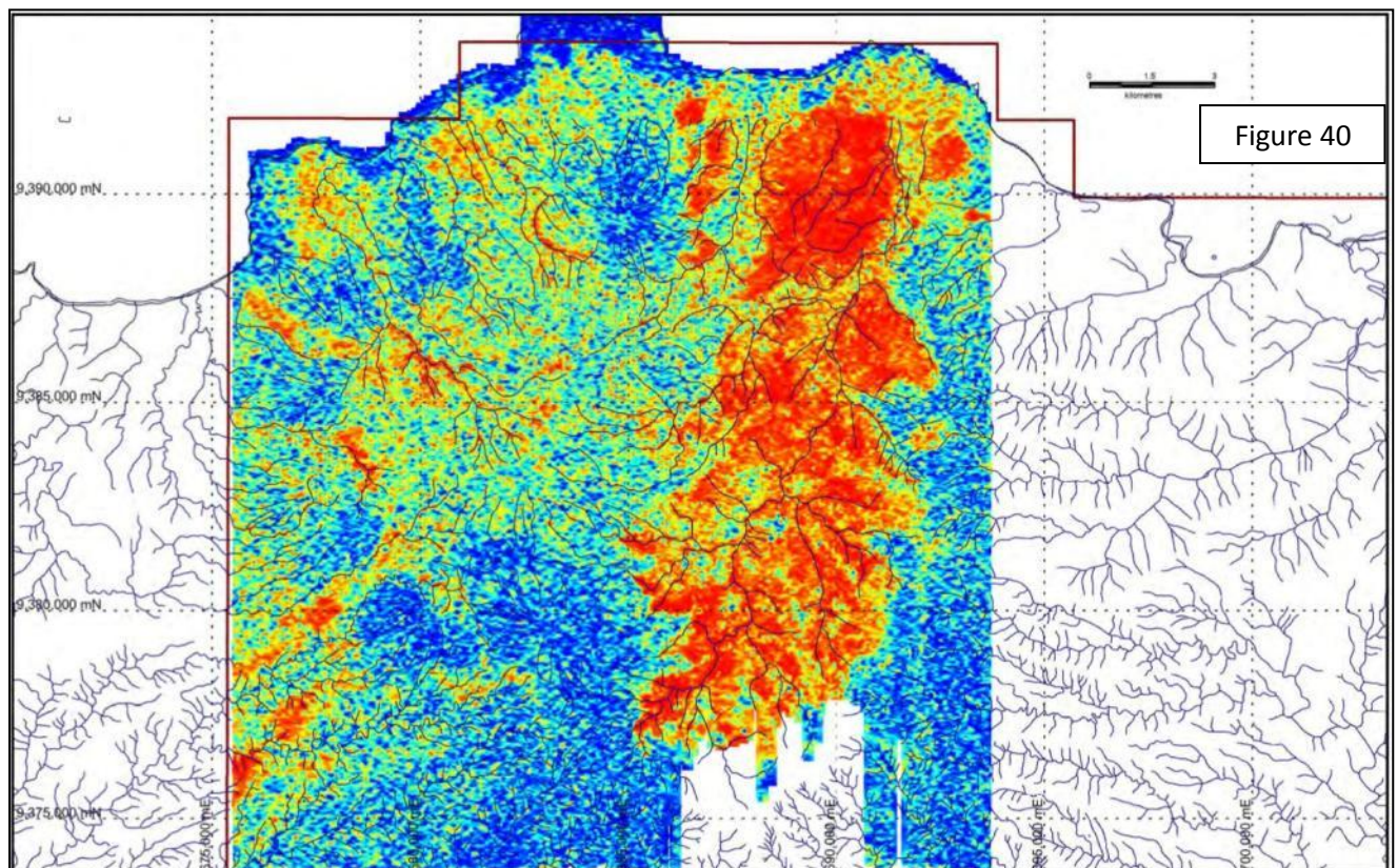
Figure 40. Uranium (shown) and Thorium are very similar and are also similar to potassium, but define a larger area of anomalism in the northern sector of the Ugurisi River valley.
