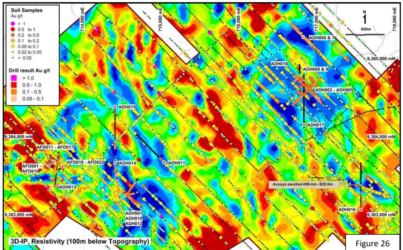
Figure 26. 3D-IP resistivity at 100m below topography showing drill hole locations and colour coded downhole gold assays.
