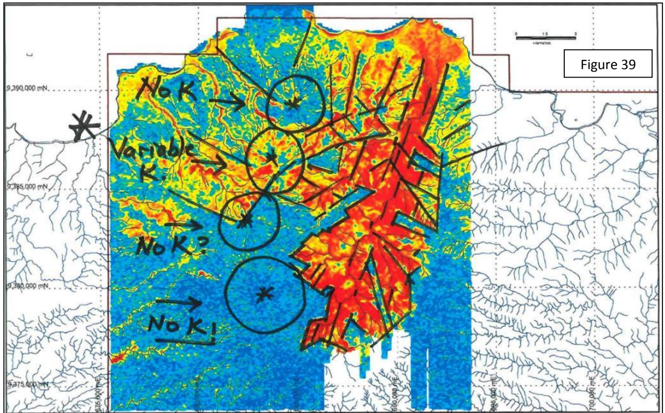
Figure 39. Strong potassium radiometrics are shown predominantly occupying the Ugurisi River valley and reflecting the major controlling NNE trending 'cross' island structure. Linear features associated with the anomaly are shown, along with the location of the volcanic cones in the western sector of the crater and a notation as to their variable potassium response.
