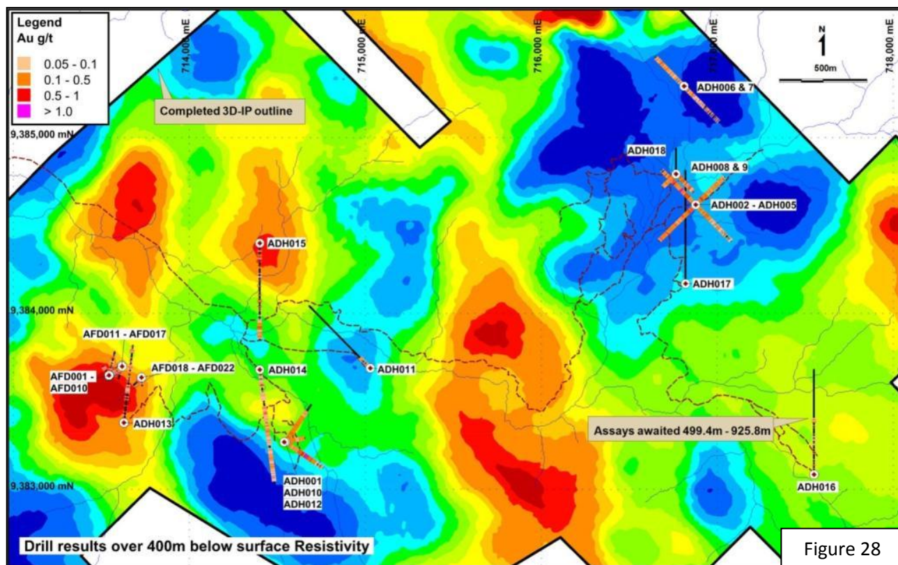
Figure 28. 3D-IP resistivity at 400m below topography showing drill hole locations and colour coded downhole gold assays.
