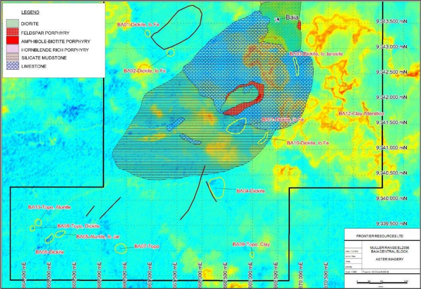
Figure 16: Baia Block Aster (Jarosite Image) with Targets
