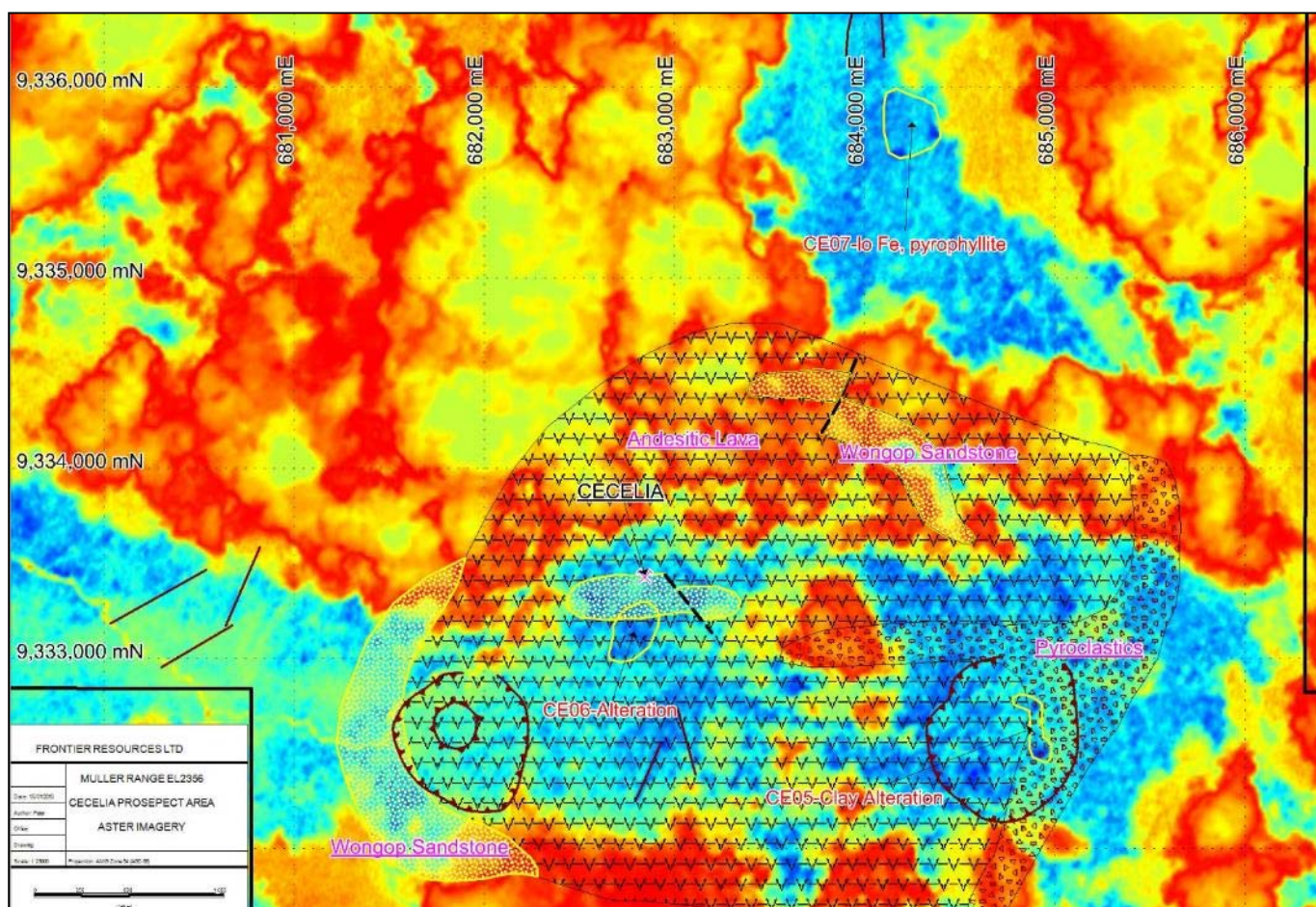
Figure 19: Cecelia North Aster (Jarosite Image) with Geology and Targets
