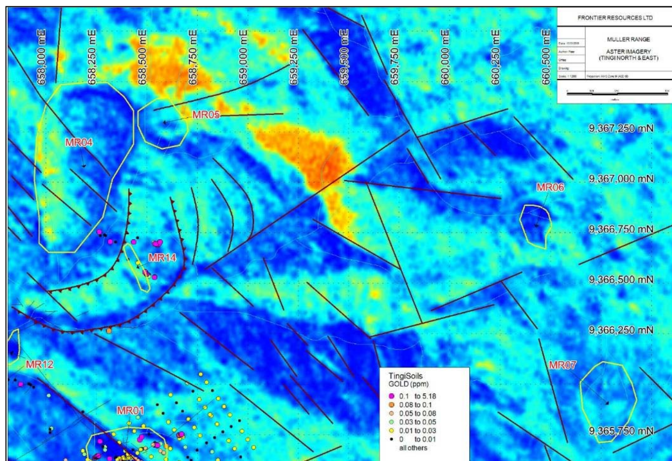
Figure 9: Tingi North Area Aster (Jarosite Image) Targets
