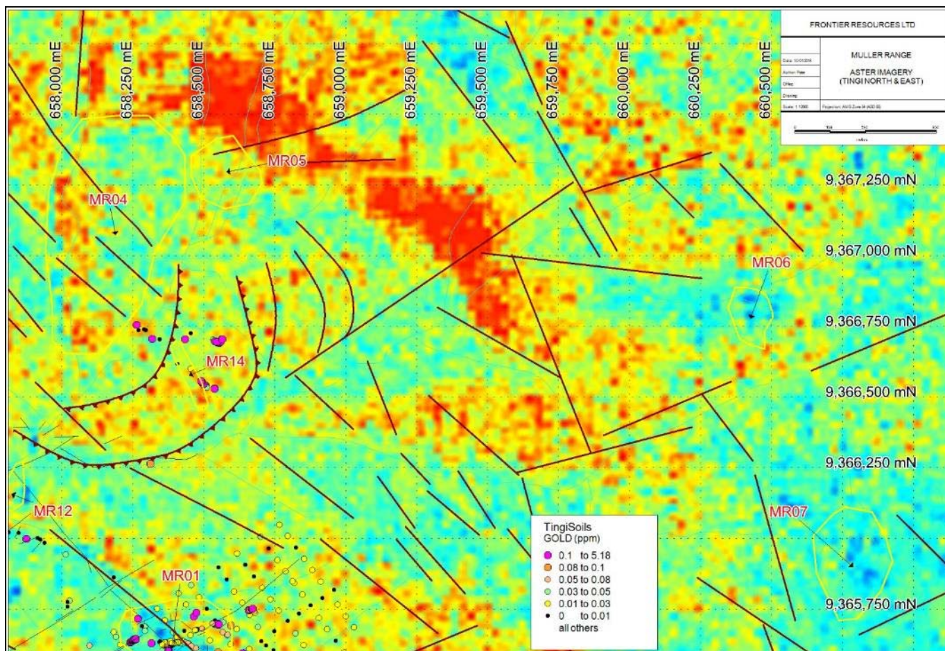
Figure 8: Tingi North Area Aster (Alunite Image) Targets
