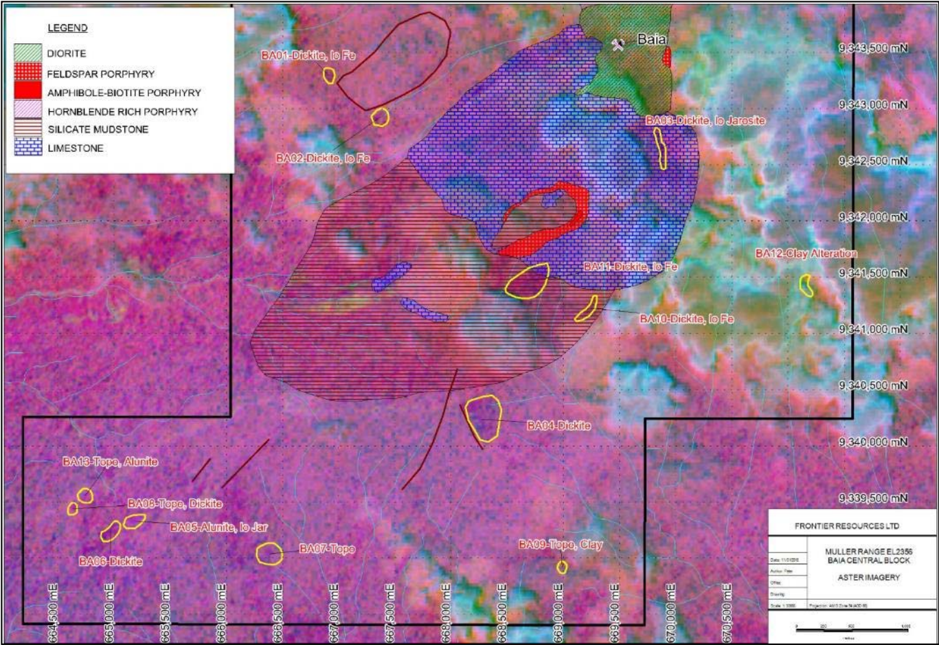
Figure 15: Baia Block Aster (Dickite-Jarosite-Pyrophyllite Image) with Targets
