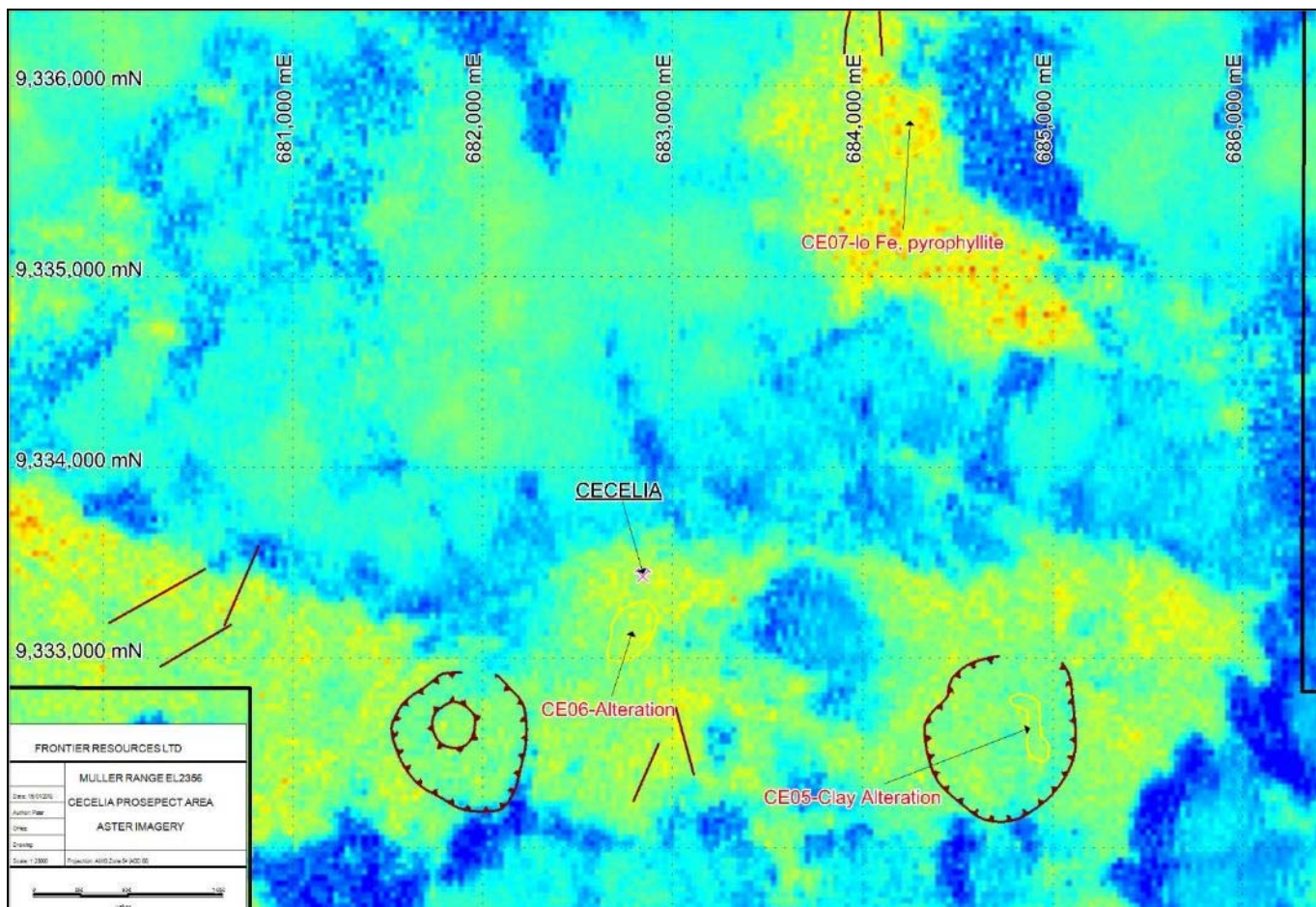
Figure 18: Cecelia North Aster (Clay Image) with Targets
