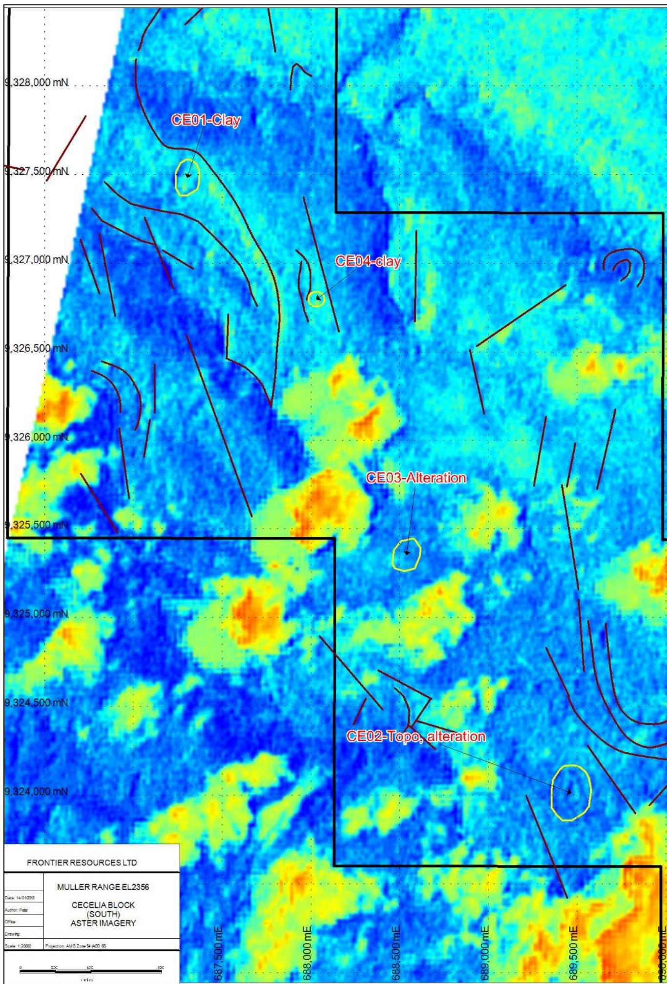
Figure 21: Cecelia South Aster (Jarosite Image) with Targets
