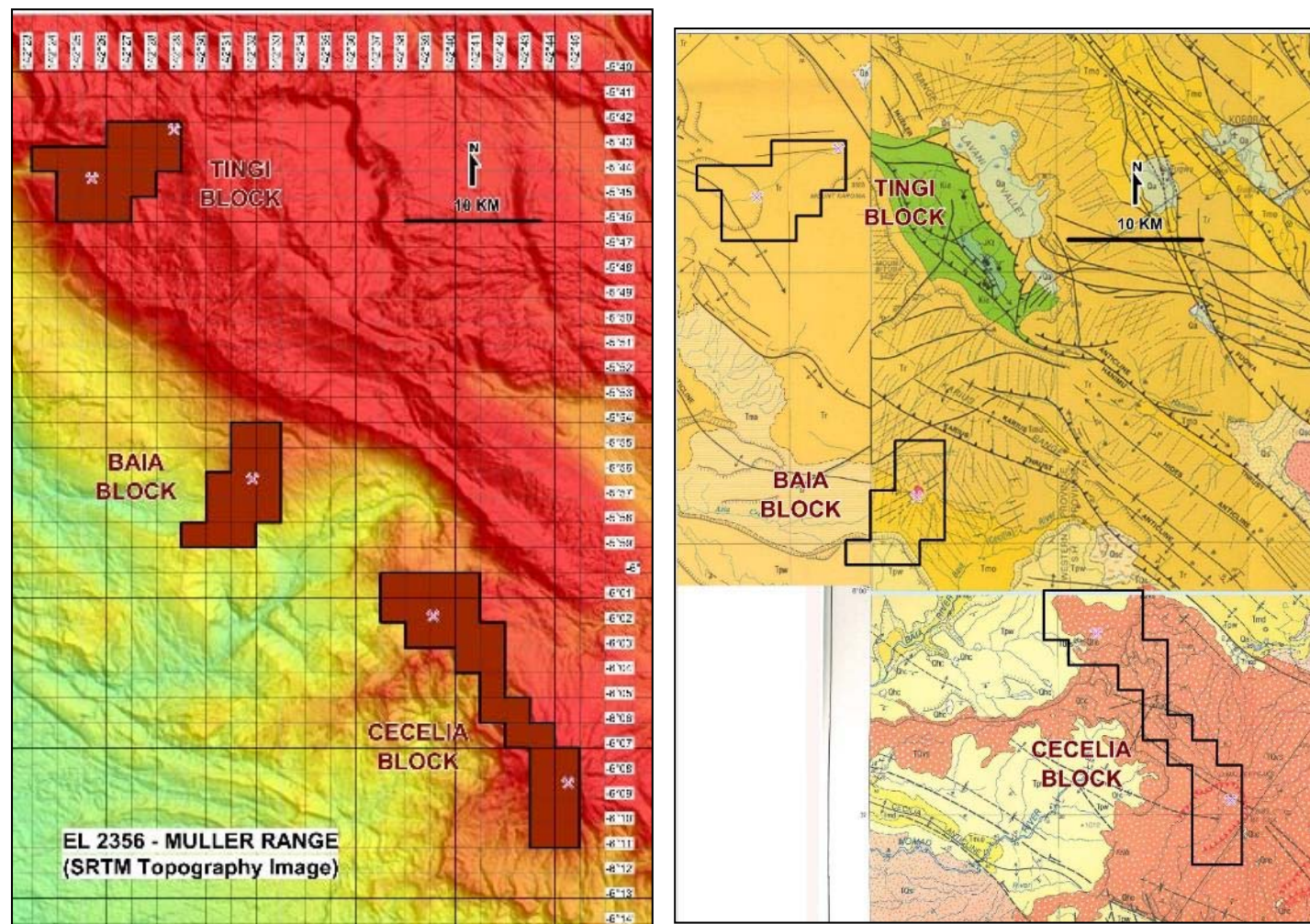
Figure 2 Location plan showing the northern Tingi Block, central Baia Block and southern Cecelia Blocks
