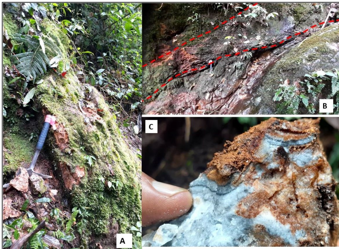
Photo 1: Kimono Central Silicified Outcrop. (A) 1m wide quartz vein along walking track; (B) 1-2m wide quartz vein near KI001 drill pad dipping into the page; (C) Epithermal textures including colloform banding with abundant dark fine grain sulphides.
