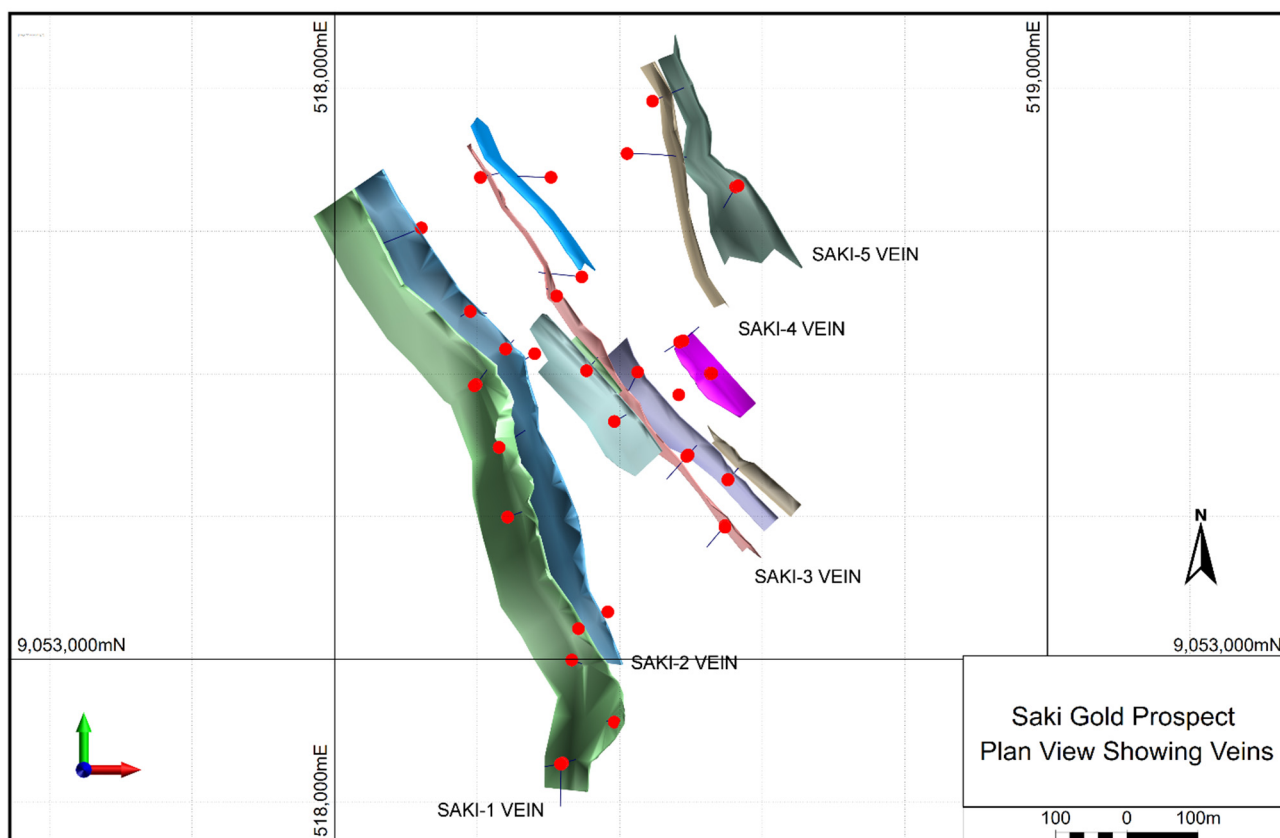
Figure 3: Saki Modelled Veins and Drillhole Locations
