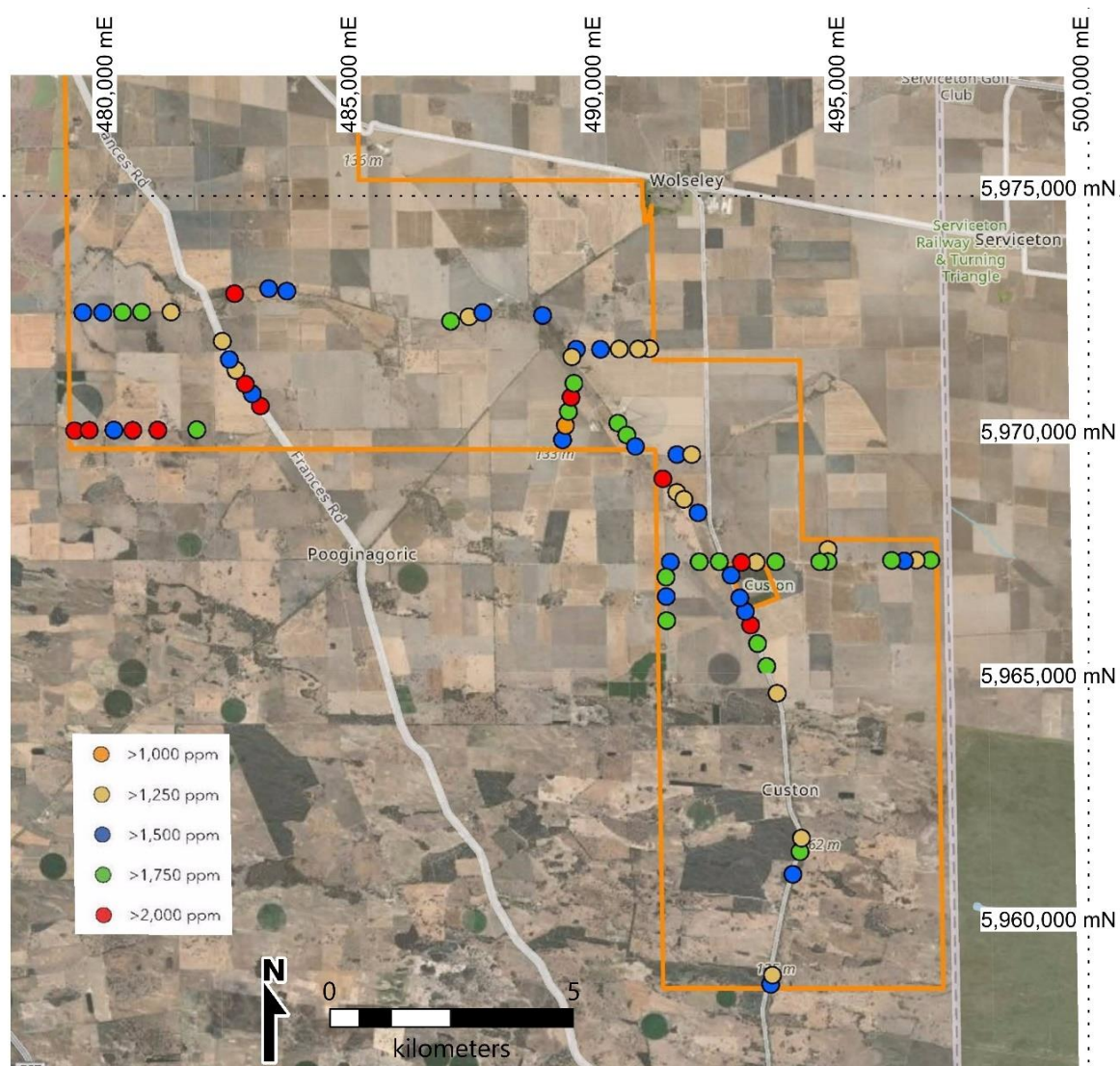
Figure 2: Locations of Roadside Air Core Drill Holes with Maximum XRF Readings for Each Drill Hole
