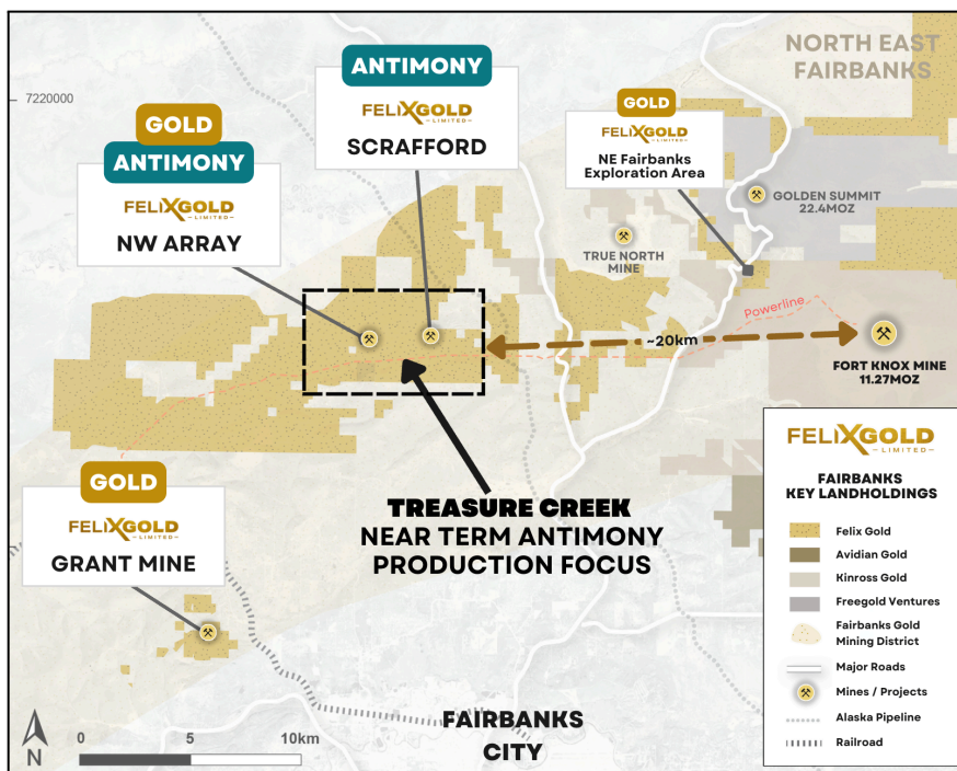
Fig 1. Location of NW Array within the Treasure Creek Antimony Project
