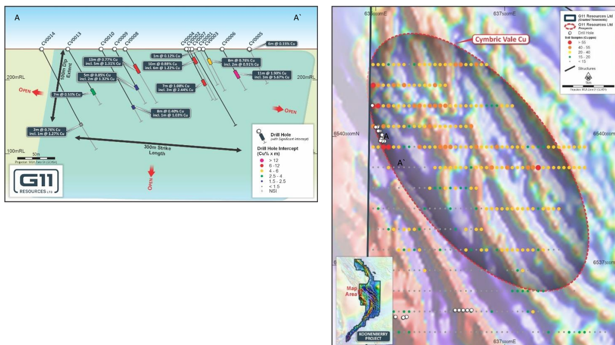
Figure 5: Oblique long section of the drill defined mineralisation at Cymbric Vale (left) and the Cu in soil geochemistry over magnetics for the broader 3km by 5km Cymbric Vale Cu prospect (right)
