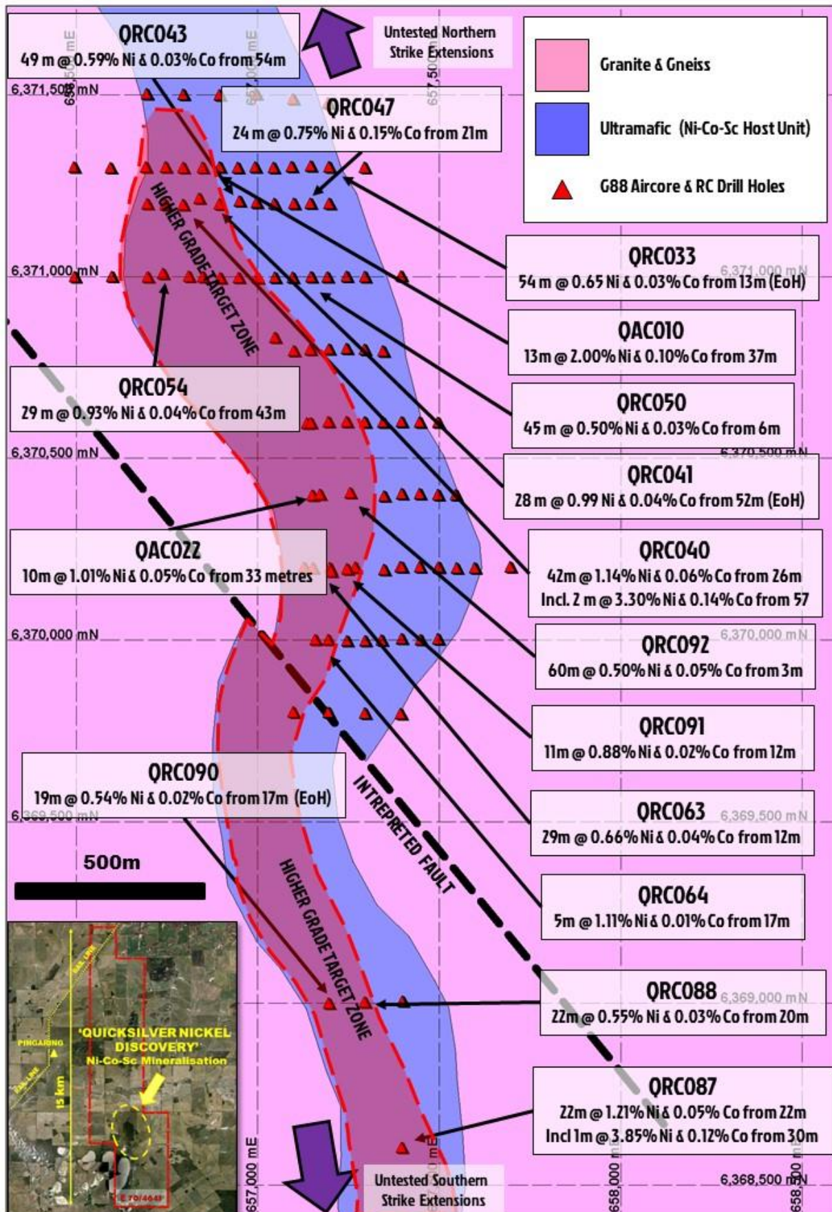
Figure 3 – Aircore & RC drill hole locations with significant nickel & cobalt intercepts over interpreted geology, with higher-grade target zone (red).
