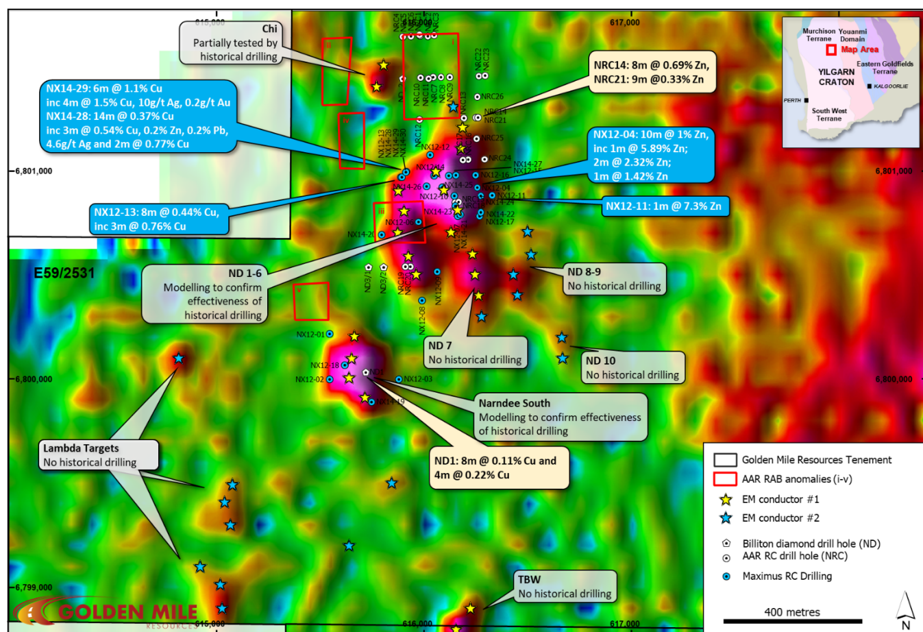
Figure 3: Yarrambee HEM survey and base metal targets with historical exploration. Background image is 25Hz base channel 23 Bfield (Z component). Refer body of text for discussion of historical work.
