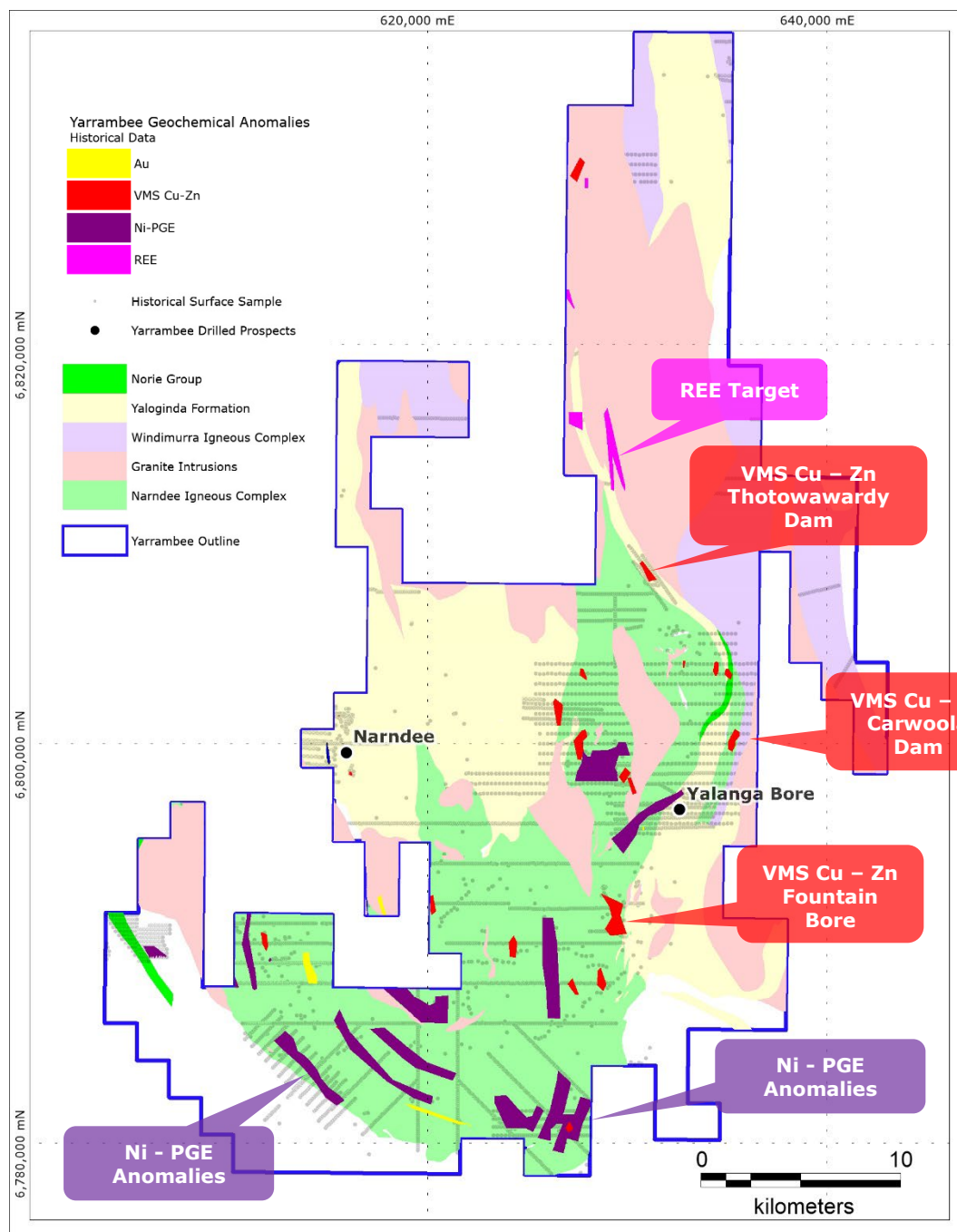
Figure 2. New Geochemical Anomalies identified in review by GCXplore Pty Ltd at Yarrabee.
