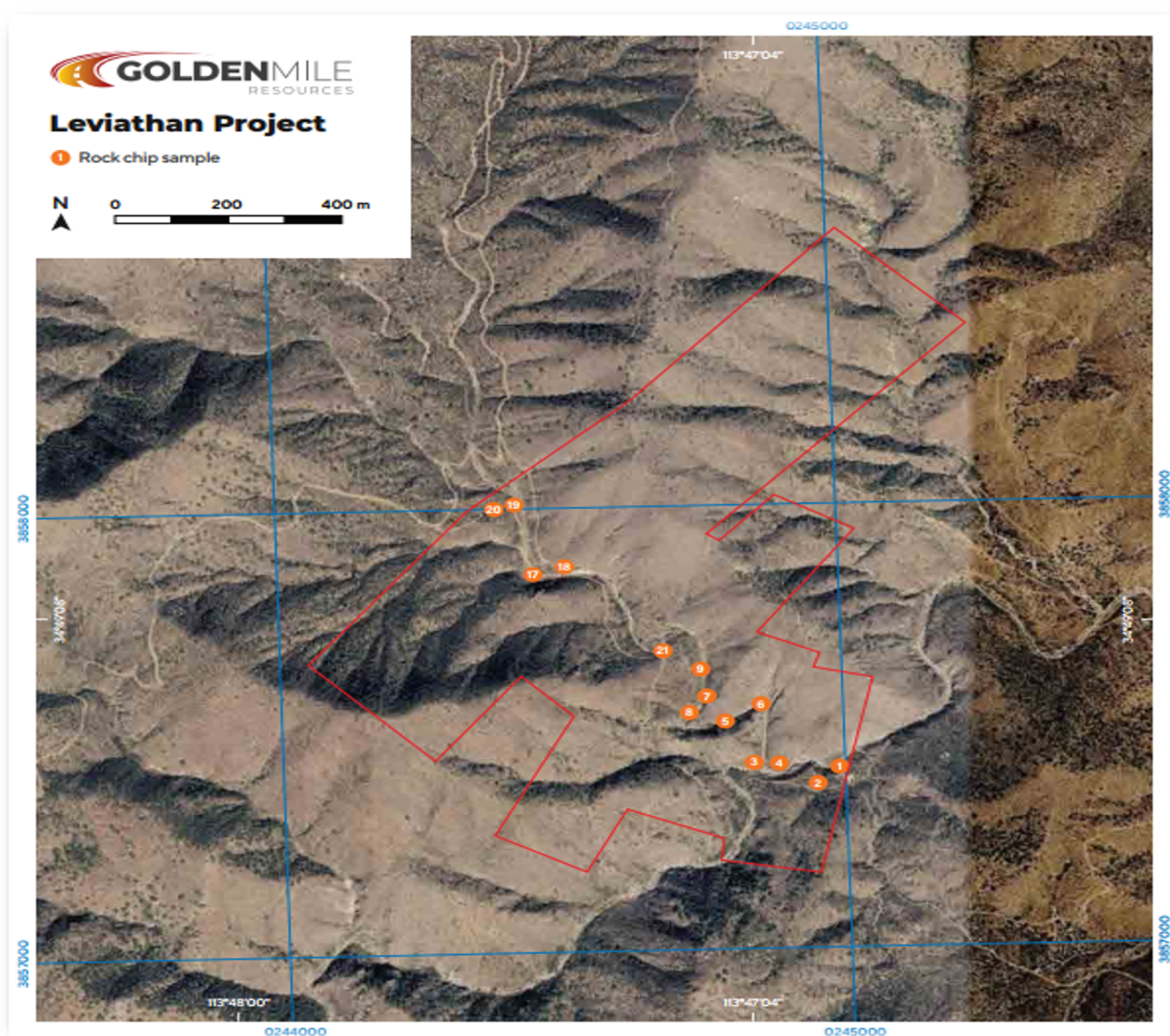
Figure 3: Leviathan Project Location Plan with sample locations and project claim boundary
