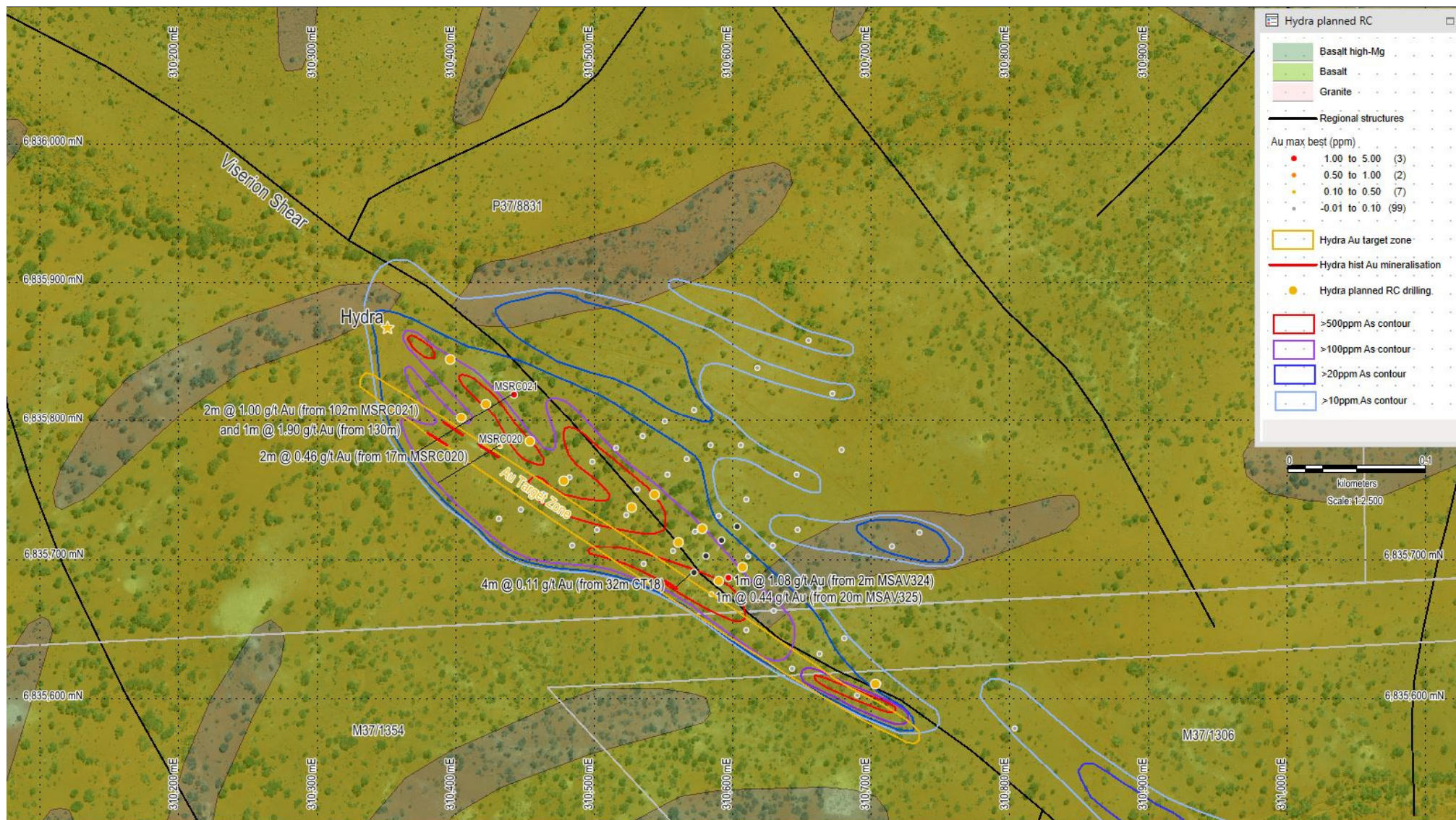
Figure 2: Hydra Au target zone and planned RC against arsenic contours on Regional Geology and structure
