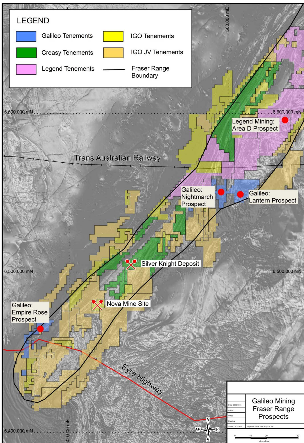
Figure 3 – Galileo's Fraser Range tenement holdings (blue) with Empire Rose, Nightmarch and Lantern prospect locations as marked. Nightmarch is 60km along strike of the Silver Knight deposit. Empire Rose is 40 km from the Nova mine site.
