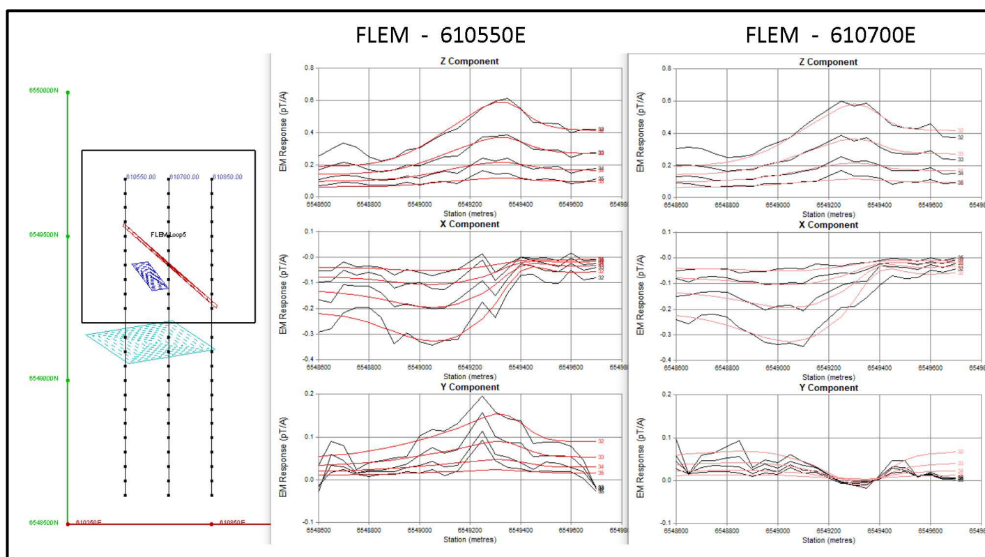
Figure 5 - New FLEM Modelling Showing Reasonable Fit to the Field Data
