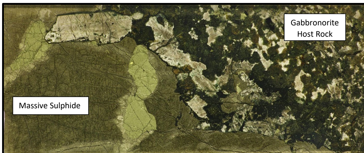
Figure 3 – Massive Pyrrhotite-Chalcopyrite-Pentlandite Sulphide Mineralisation in Lantern South Diamond Drill Core (scale: height of slide = 26mm, from 136.2m downhole, LARC013D)
