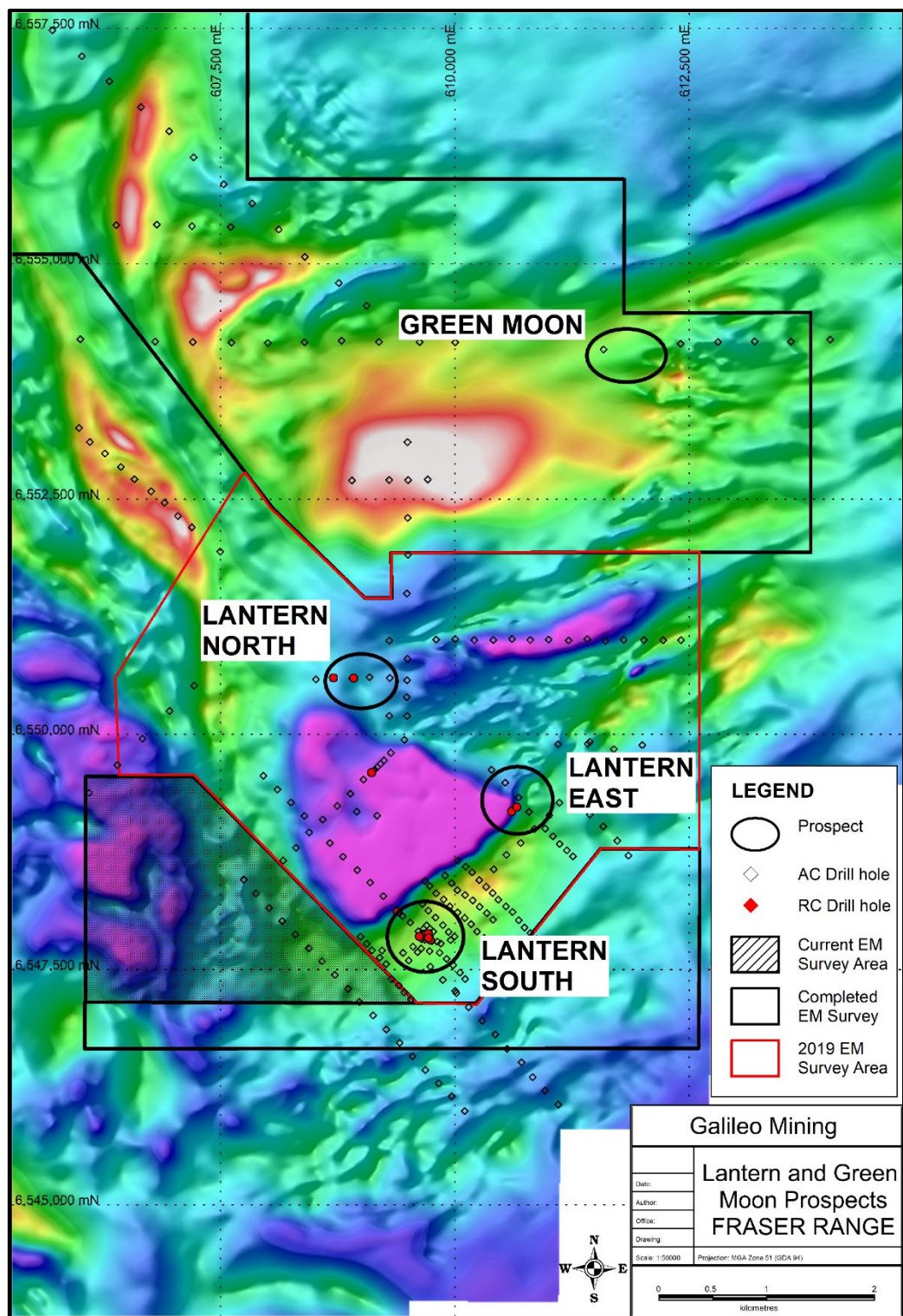
Figure 2 – EM Surveying and Prospect Locations Surrounding Galileo's Lantern Prospect in the Fraser Range (TMI magnetic background imagery)
