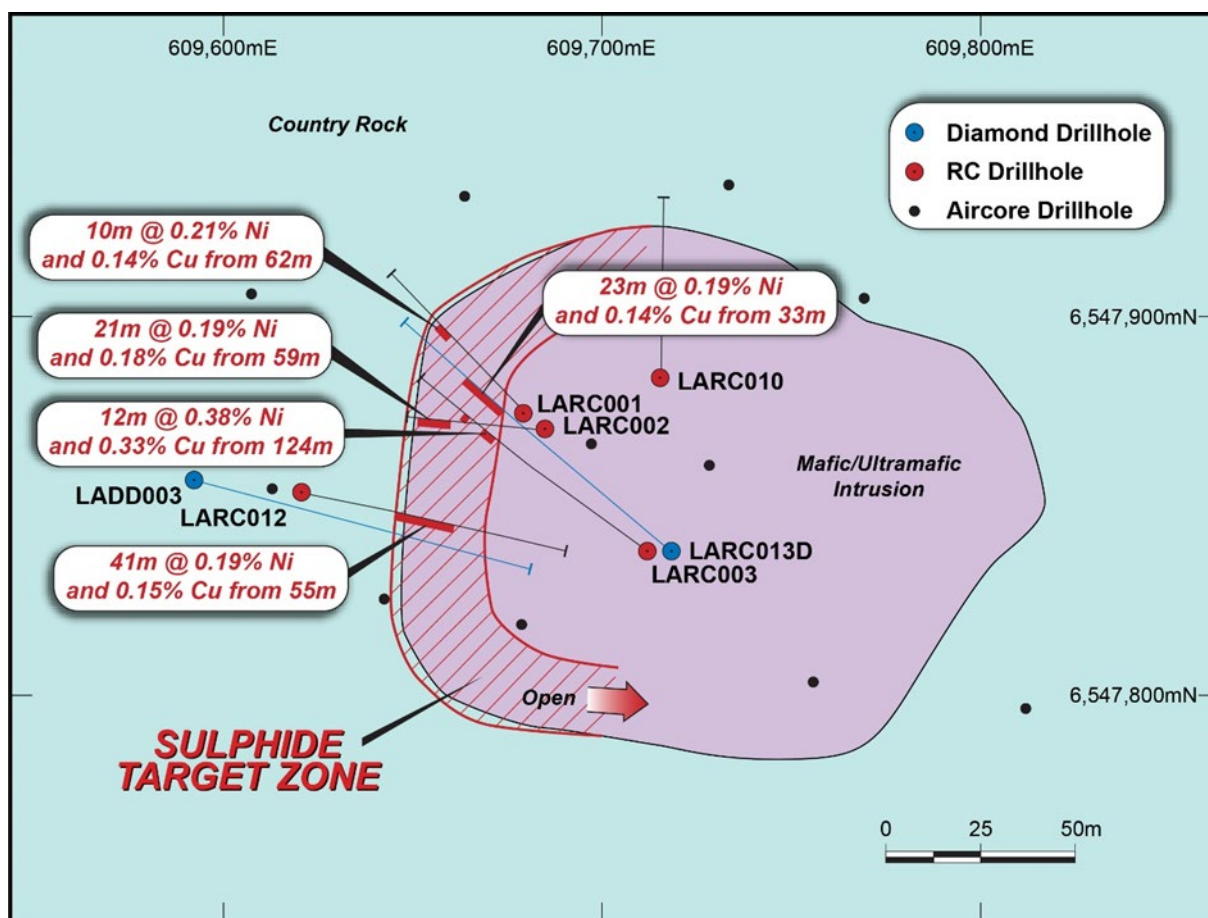
Figure 2 —Lantern South Prospect Plan Showing Sulphide Target Zone and Drill Hole LADD003
