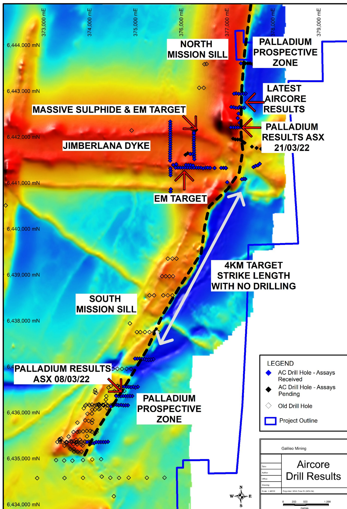
Figure 2 — Location of aircore drilling over the Mission Sill and the Jimberlana Dyke. Palladium prospective zone with untested 4km strike length as marked. Magnetic background is TMI.
