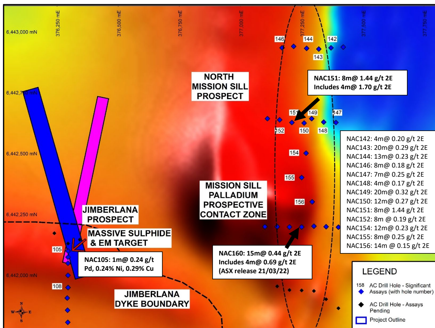
Figure 1 — Location of northern Mission Sill aircore drilling with anomalous palladium for selected drill holes. 2E = palladium + platinum, see Table 1 for full details. TMI magnetic image in background.
