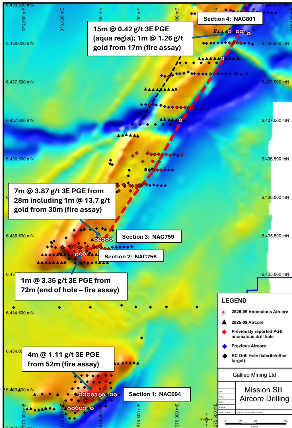
Figure 1 – September 2025 anomalous aircore drill results from the Mission Sill prospect with updated one split sample results. Red dashed line is the Eastern Contact target zone which now covers over 10km of strike. See Appendices for assays & details of drill holes reported in this announcement. TMI background image.
