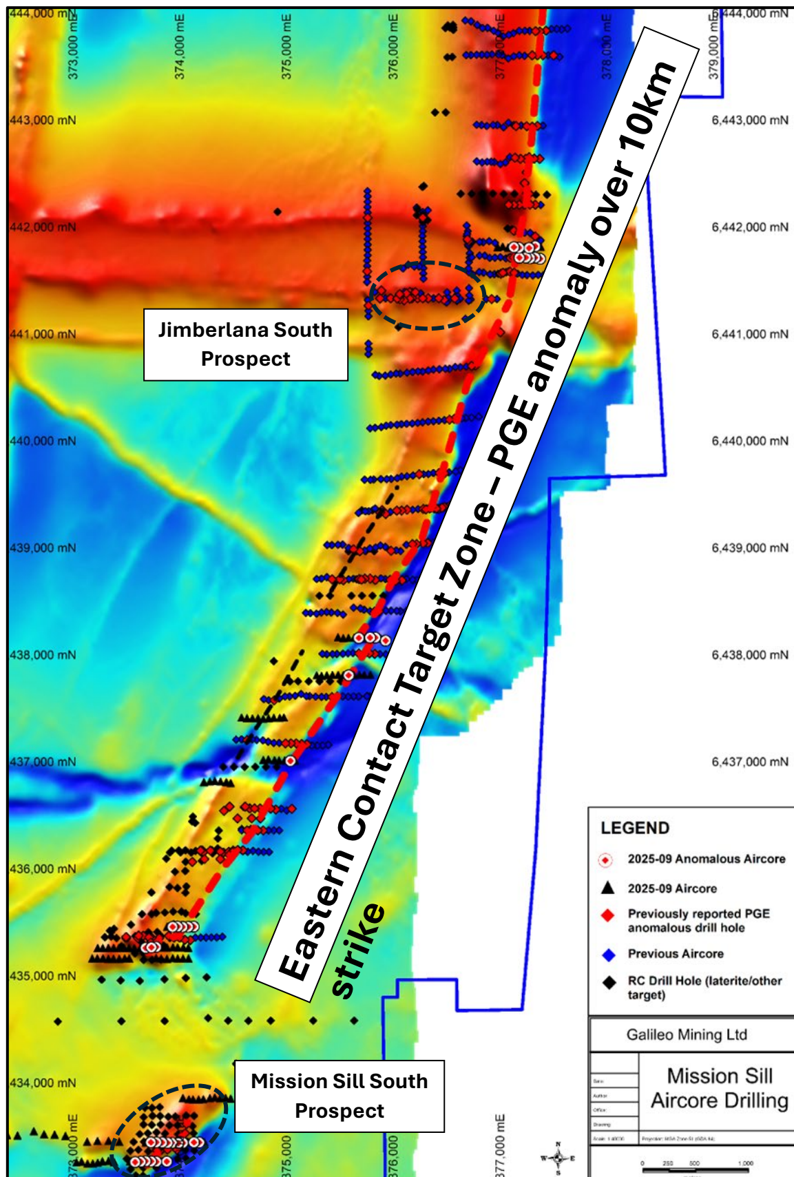
Figure 2 – Drilling at the Mission Sill prospect showing over 10km of anomalous PGE results along the Eastern Contact Zone target. Location of the Jimberlana South and Mission Sill South prospects also shown. TMI magnetic background image. See ASX announcement dated 8/09/2025 for assays and details of September anomalous aircore results.
