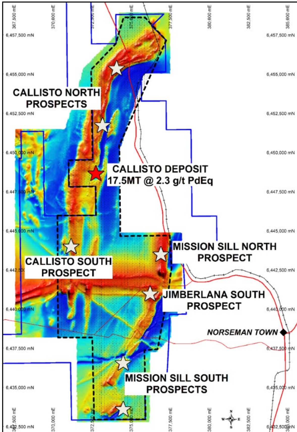
Figure 7 – Norseman Project outline (blue line) with PGE prospective area (black dashed line), Callisto Deposit (red star), and prospects (grey stars).
