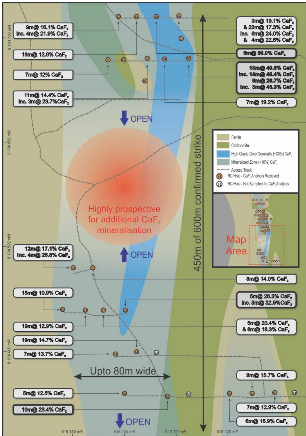
Fig 2: Main Fluorite/REE Zone drillhole location plan showing selected \text{CaF}_2 results.
