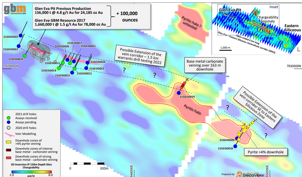
Figure 3. 2021 and 2020 GBM drilling at Glen Eva and geophysical targets 1.5 km to the southeast overlain on a 150 m IP chargeability depth slice. Also shown are modelled veins and the Glen Eva pit, 21GEDD018 and 21GEDD020 “pyrite halo” and 21GEDD019 down hole interval of carbonate base metal veining.
