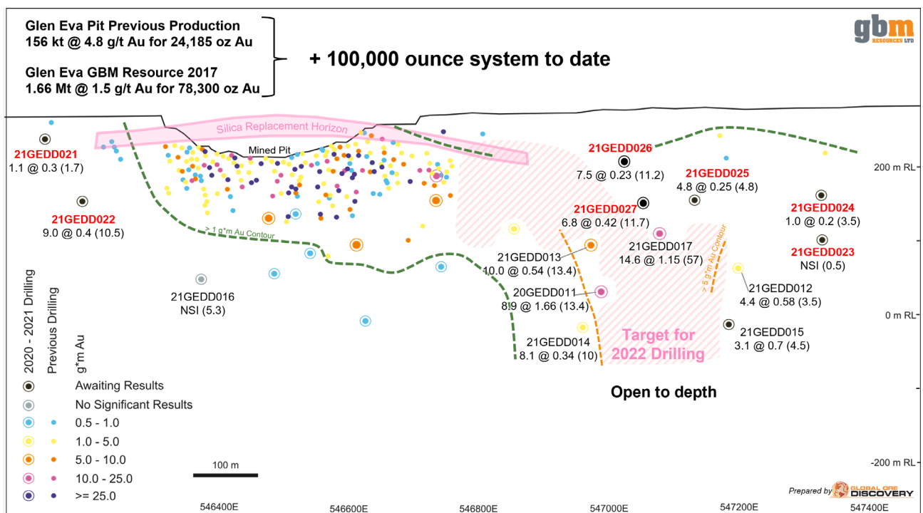
Figure 1. A long section along the Glen Eva vein showing recent 2021 drilling and g*m intercepts. Note that the vein has now been intercepted over more than 1 km of strike. Assay results and vein widths are shown underneath the hole ID's with intervals in metres and gold grades in g/t Au. Down hole vein zone widths in metres are in the parentheses. Note that the best intercepts of the 2021 program correspond to the greatest vein widths and define a steeply plunging shoot.
