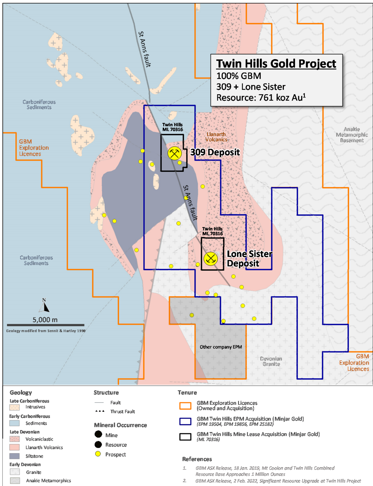
Figure 6: Geological setting of 309 and Lone Sister Deposits
