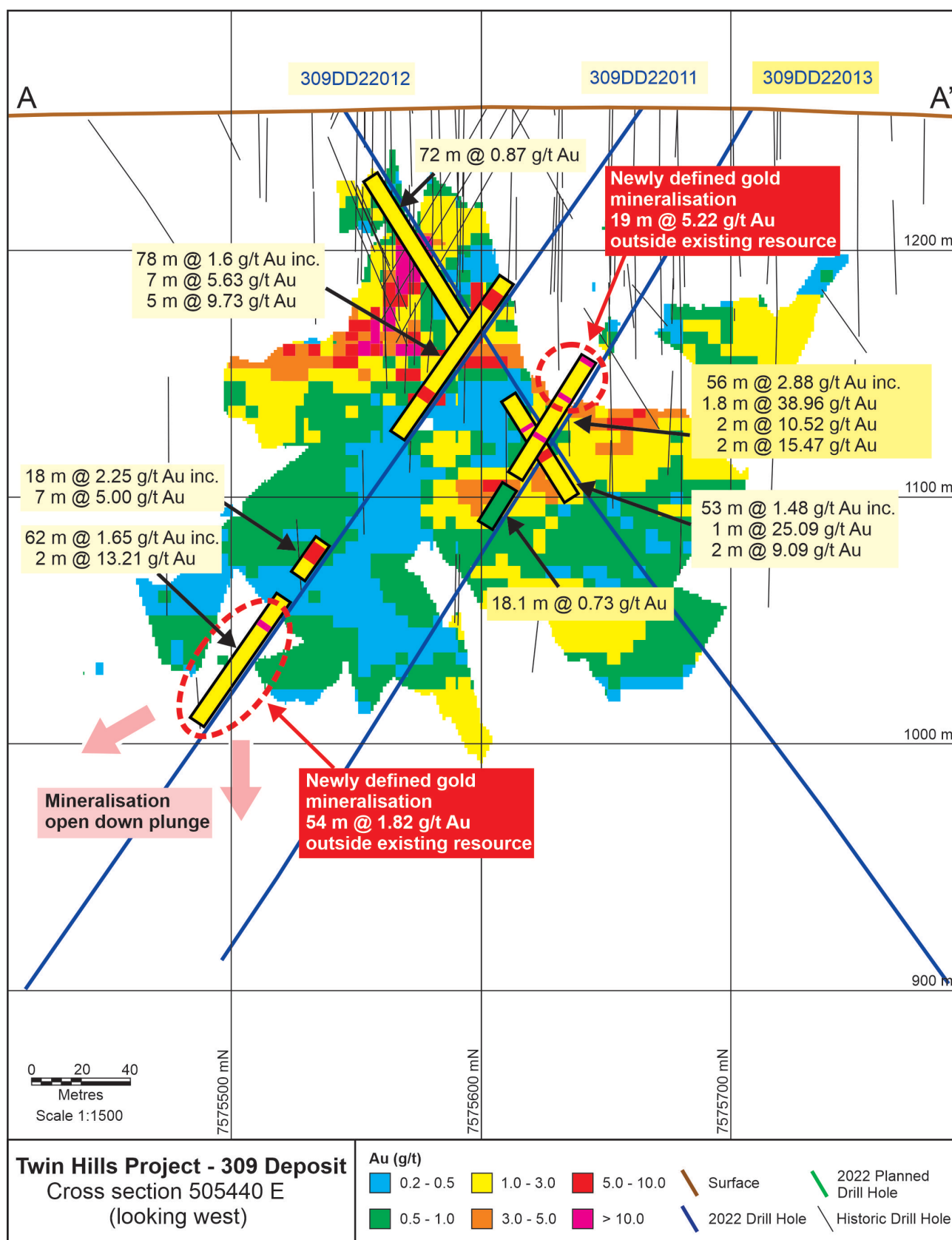
Figure 2: A cross-section (A-A') showing assay results for drill hole 309DD22013 and recently reported drill holes 309DD22011 and 012 (Refer ASX: GBZ release 14 June 2022). Only assays with a g*m Au value of > 10 are shown. Block model block grades from the 2022 resource update (Refer ASX: GBZ release 2 February 2022) and historic drill holes are also shown.
