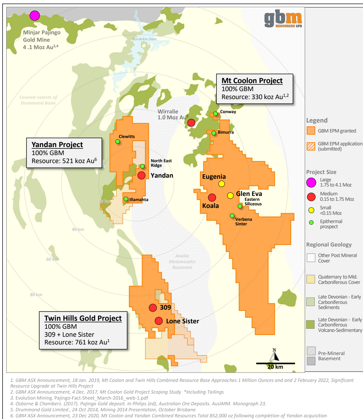
Figure 5: A map showing the distribution of GBM's tenements in the Drummond Basin. Note the location of Twin Hills 309 and Lone Sister deposits.
