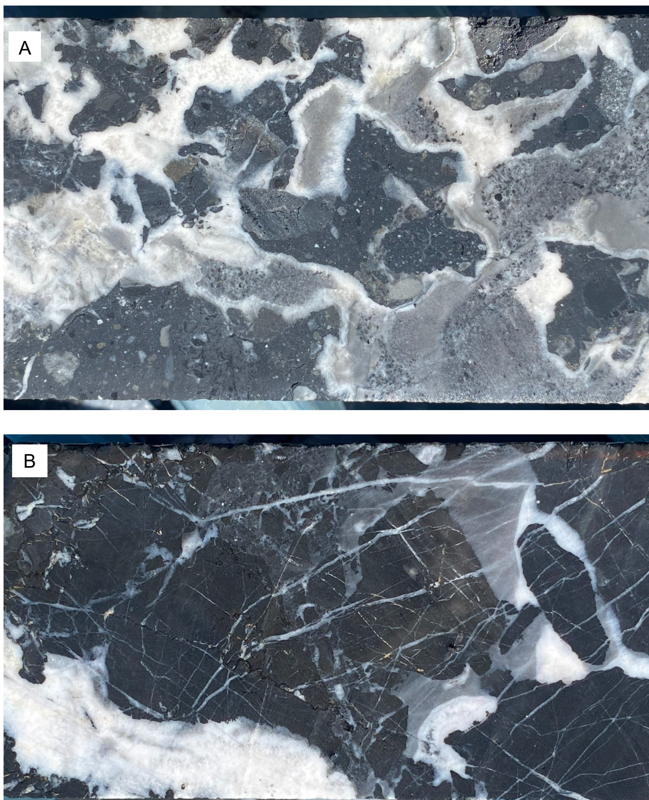
Figure 4: Photographs of drill core showing (A) Quartz-chalcedony- breccia fill hosted by milled matrix breccia at 121.9 m in 309DD22013. The interval assayed at 1.1 m @ 60.61 g/t Au from 121.7 m and (B) Multi-stage quartz-chalcedony veins and breccia fill at 262.6 m in 309DD22014. The interval assayed at 1 m @ 5.12 g/t Au.
