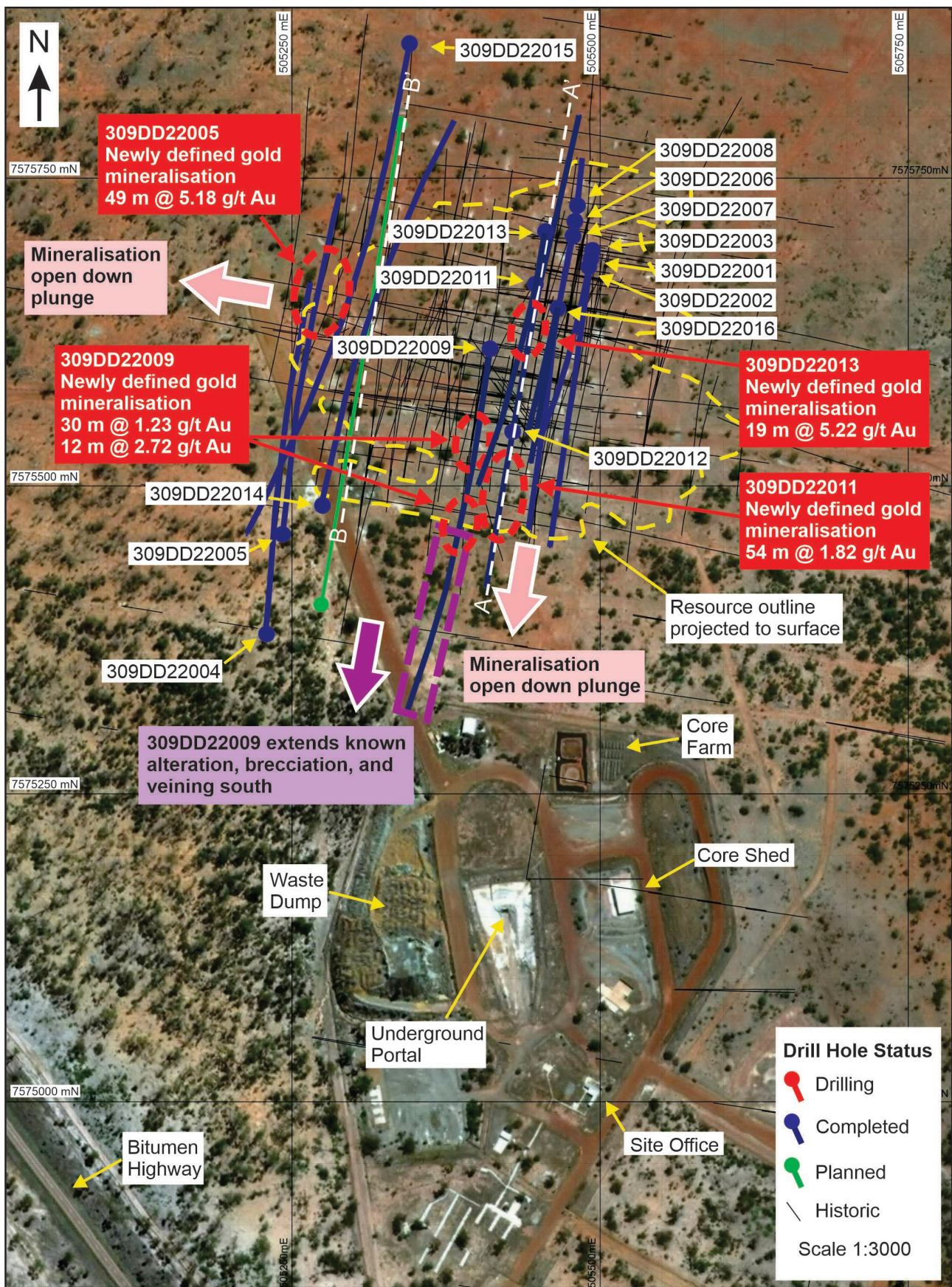
Figure 1: A map showing the location of recently completed and proposed drill holes at the 309 Deposit. Note the location of section line A-A' for Figure 2 and B-B' for Figure 3. Also shown is established infrastructure, block model outline projected to surface and historic drill holes.
