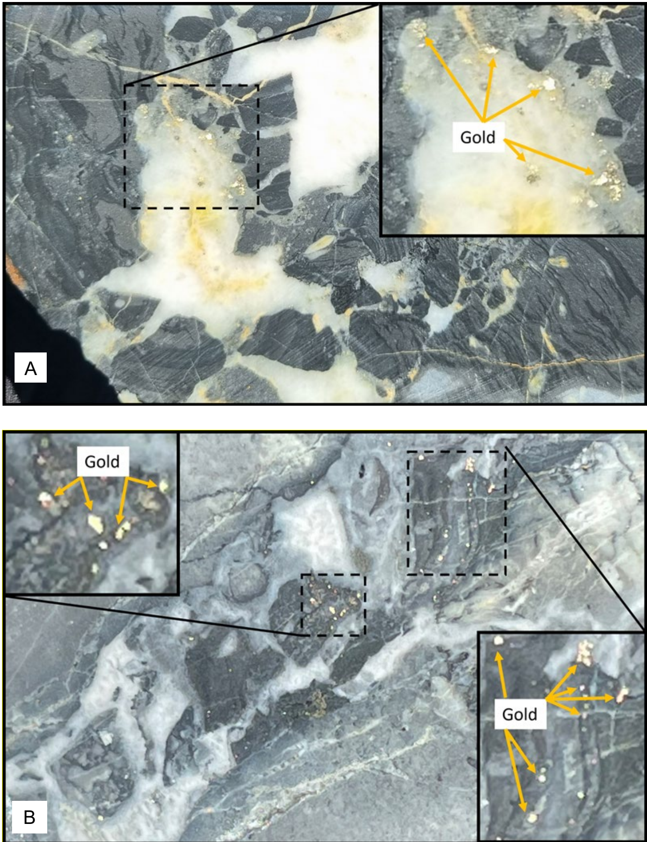
Figure 4: Photographs of drill core showing (A) Quartz-chalcedony-illite breccia fill with visible gold hosted by siltstone at 426.6 m in 309DD22015. The interval assayed at 1.0 m @ 42.01 g/t Au from 426 m and (B) Multi-stage quartz-chalcedony-pyrite breccia vein with visible gold at 287.8 m in 309DD22016. The interval assayed at 0.5 m @ 166.05 g/t Au. Field of view width of main photos approx. 50 mm.
