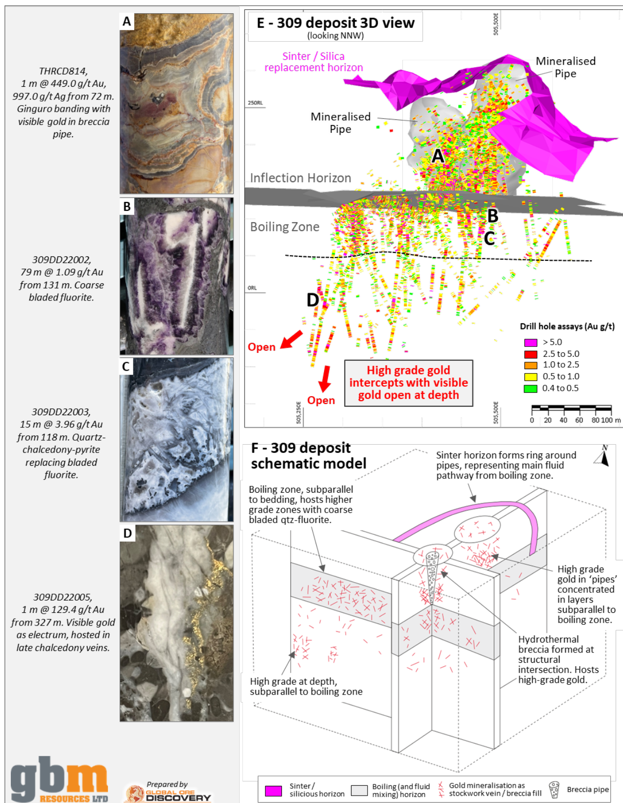
Figure 4: 309 Deposit mineralisation model. 4 A – D show variation in mineralisation styles across the deposit with sample locations shown on 4 E. Abundant bladed fluorite and fluorite replaced by silica forms in a distinct zone that we interpret to result from boiling. The fluorite-rich boiling zone marks an inflection point in deposit geometry above which mineralisation forms two pipe-like bodies along a NNE trend (4 E and F). Note that elevated gold grades form
