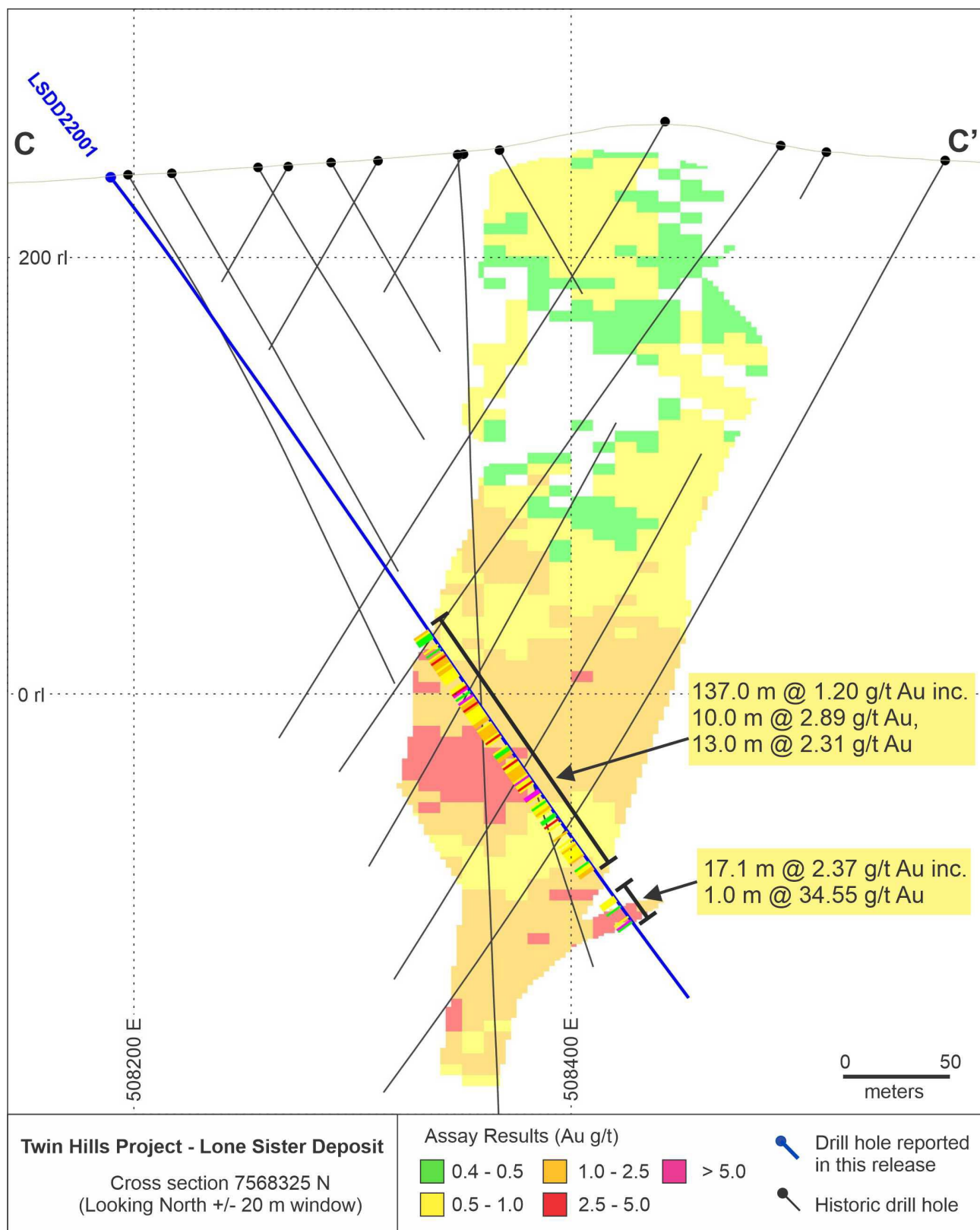
Figure 6: A cross-section (C-C') showing assay results for drill hole LSDD22001 overlain on the 2022 block model and historic drill holes.
