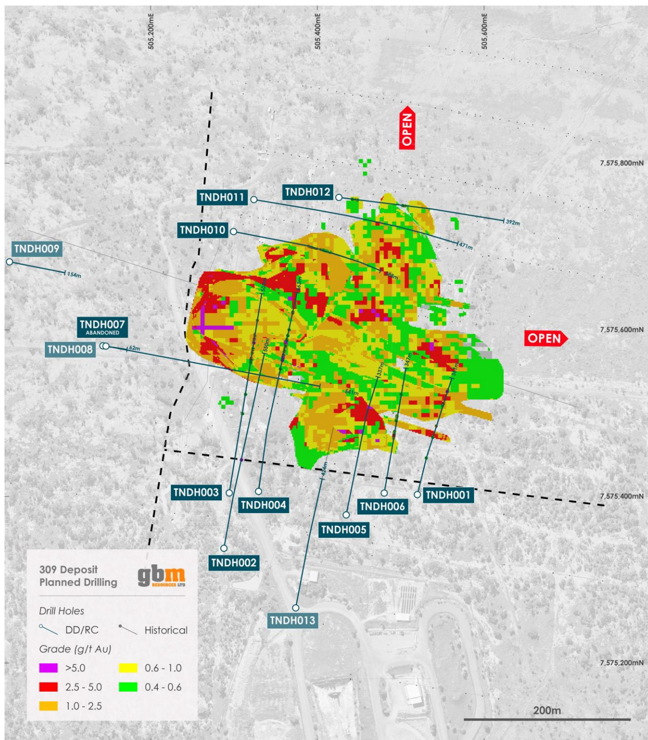
Figure 4 – Plan view of the Stage 1 holes drilled at the 309 deposit.
