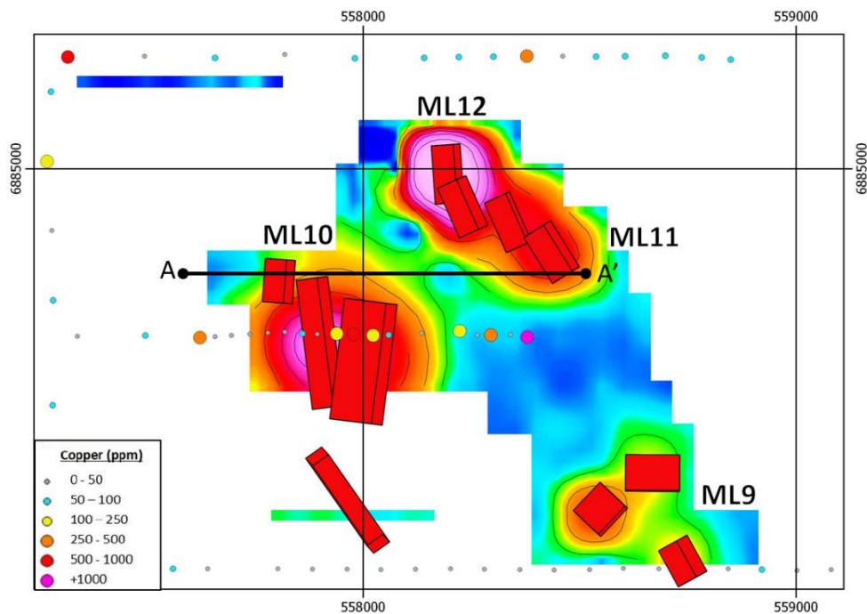
Figure 2A: Plan view map of intersection of the eastern shear zone with the core of the intrusion showing Ch 35 MLEM image and modelled conductor plates with end of hole (fresh rock) copper aircore geochemistry 1
