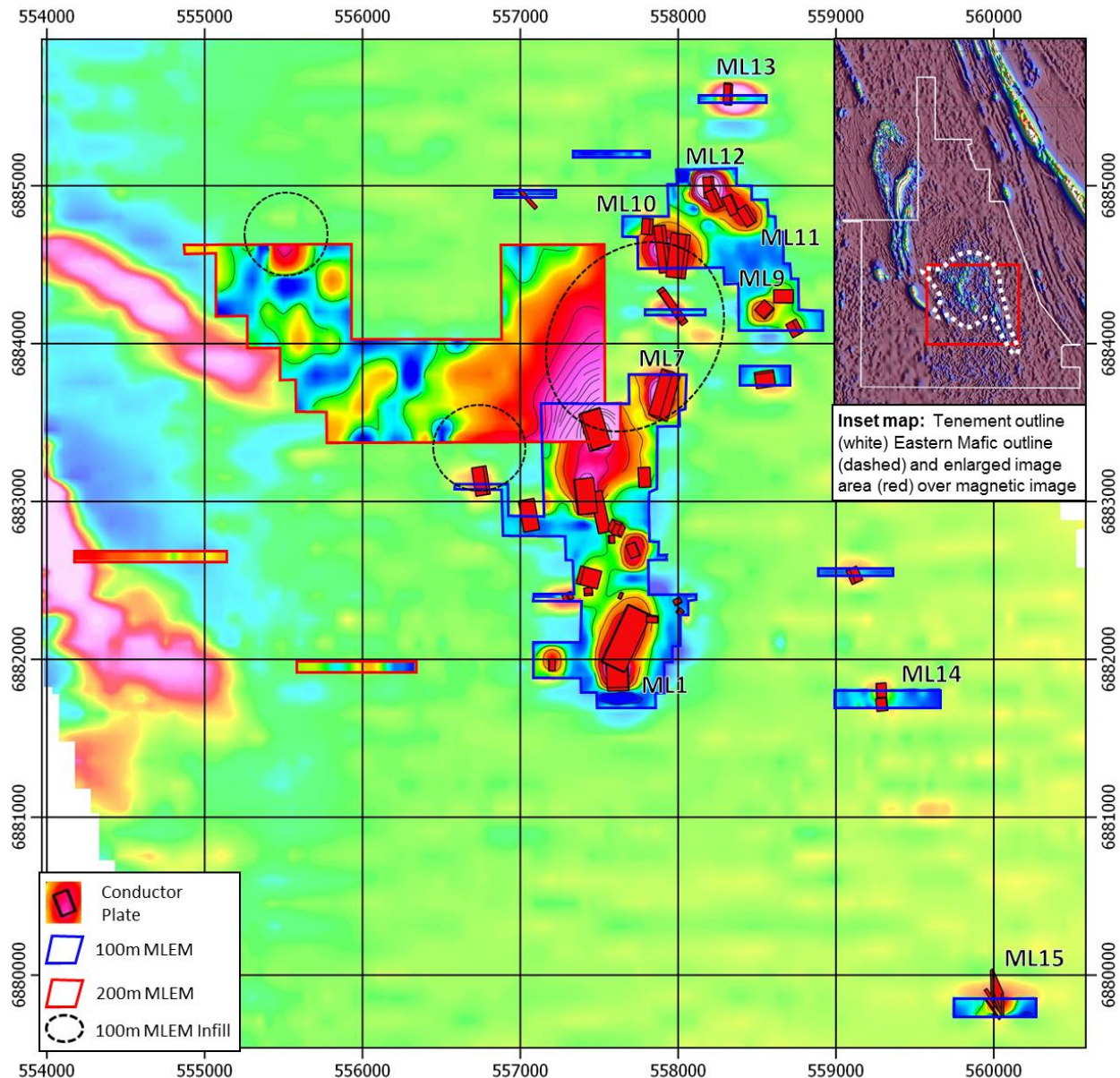
Figure 1: MLEM late time (Ch. 35) showing 100m loop survey (blue) and 200m loop survey (red) with planned 100m loop infill areas (dashed black). Modelled conductor plates are shown in solid red: Base image late-time (Ch. 35) airborne EM
