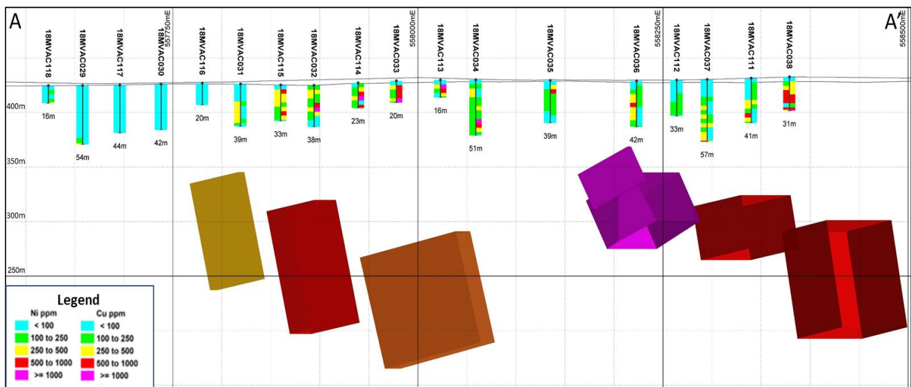
Figure 2B: X-section (6884800mN) showing conductor plate depth and orientation with overlying copper-nickel supergene mineralisation from aircore geochemistry 1 (200m window north and south from section line)
