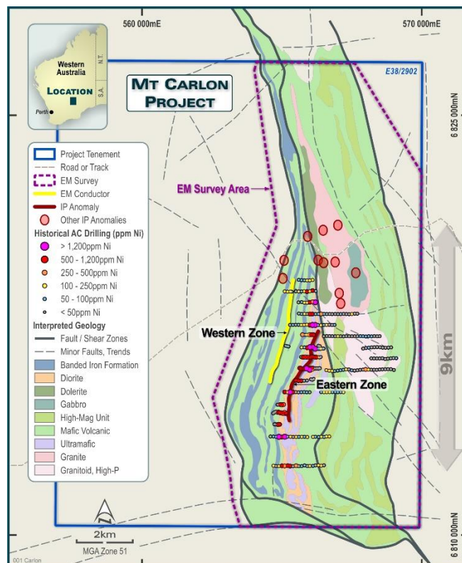
FIGURE 2: THE EASTERN ZONE IS A 3.5KM-LONG ANOMALY COINCIDENT WITH ELEVATED NICKEL IN ULTRAMAFIC ROCKS.
