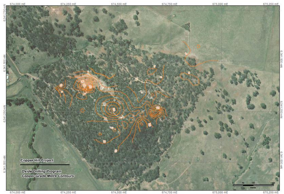
Copper Hill: Copper grade % times thickness contours
