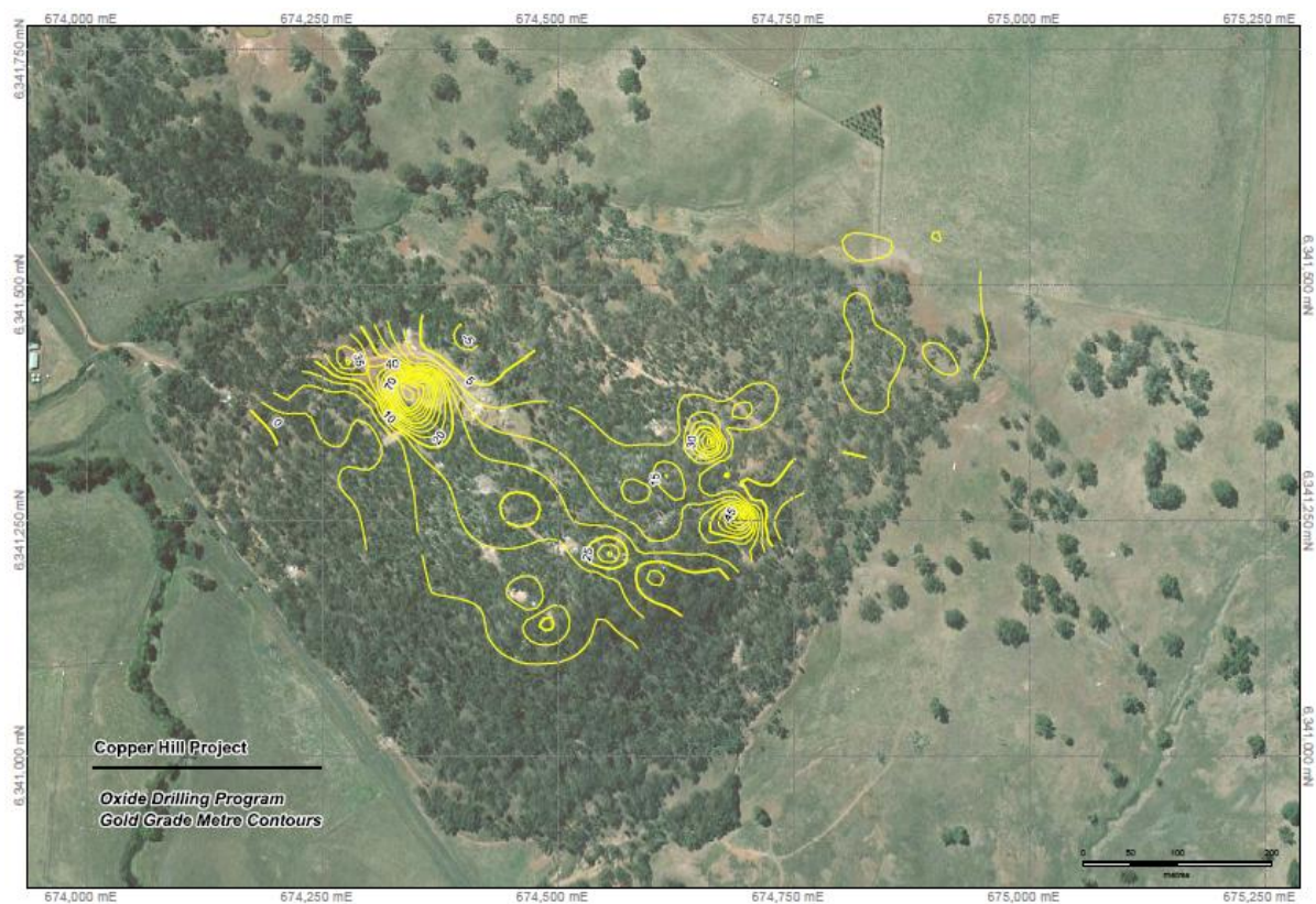
Copper Hill: Gold grade (grams/tonne) times thickness contours
