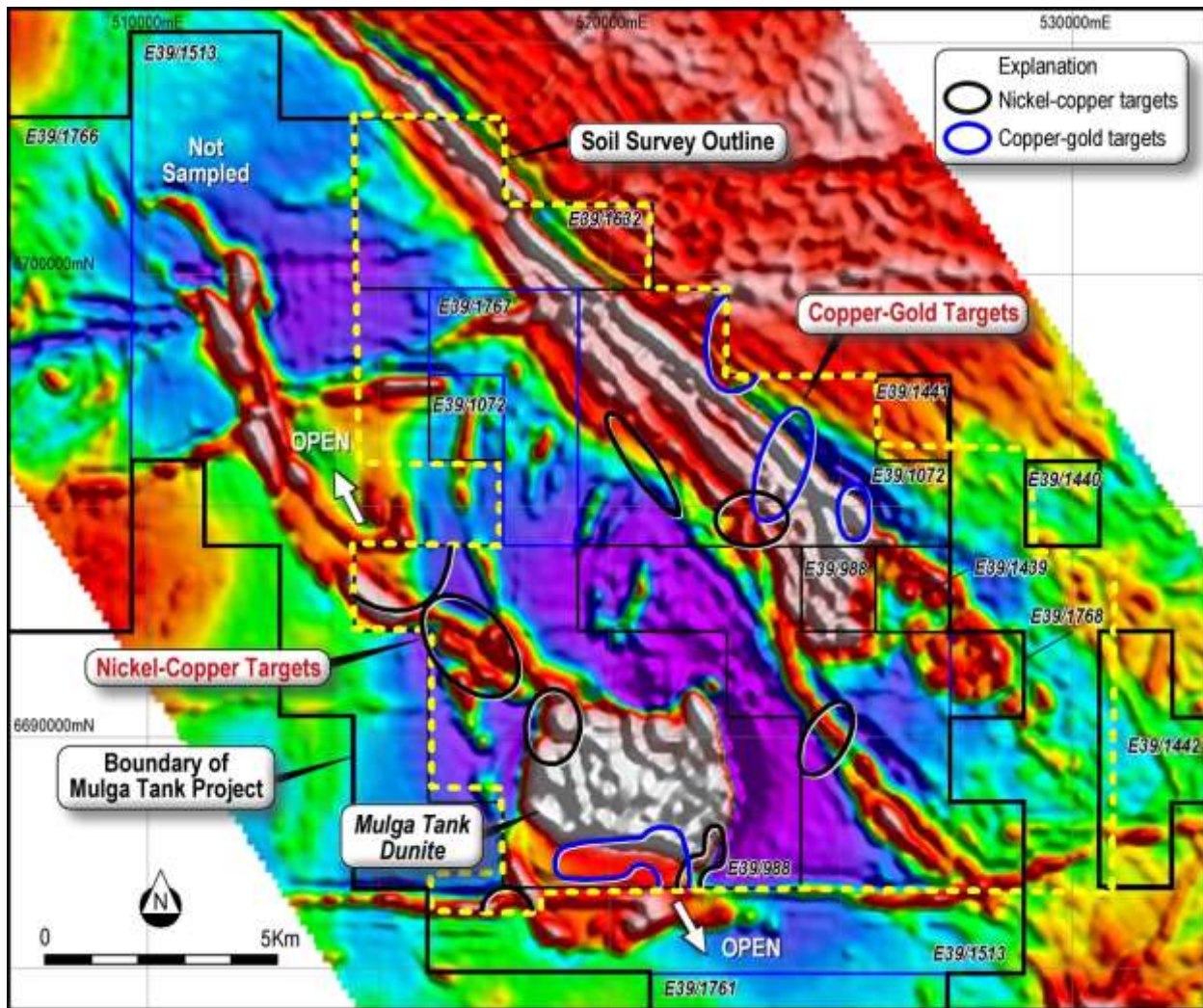
Figure 2. Image of magnetic data over the Mulga Tank Project showing the location of the new targets identified in the soil geochemistry data.
