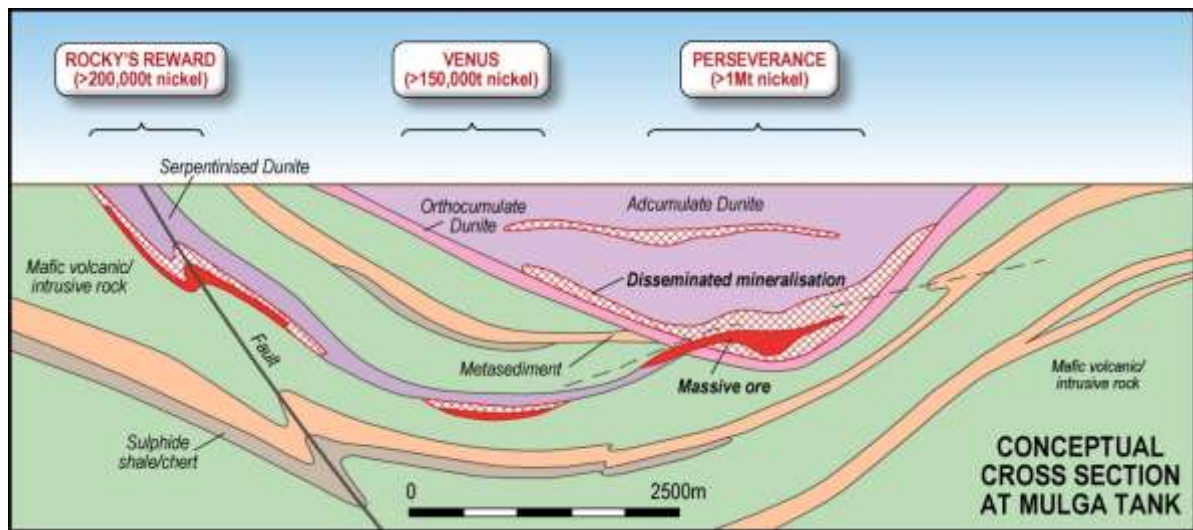
Figure 5. Conceptual cross-section for the Mulga Tank Dunite and surrounding area showing the Perseverance and Rocky's Reward exploration model.
