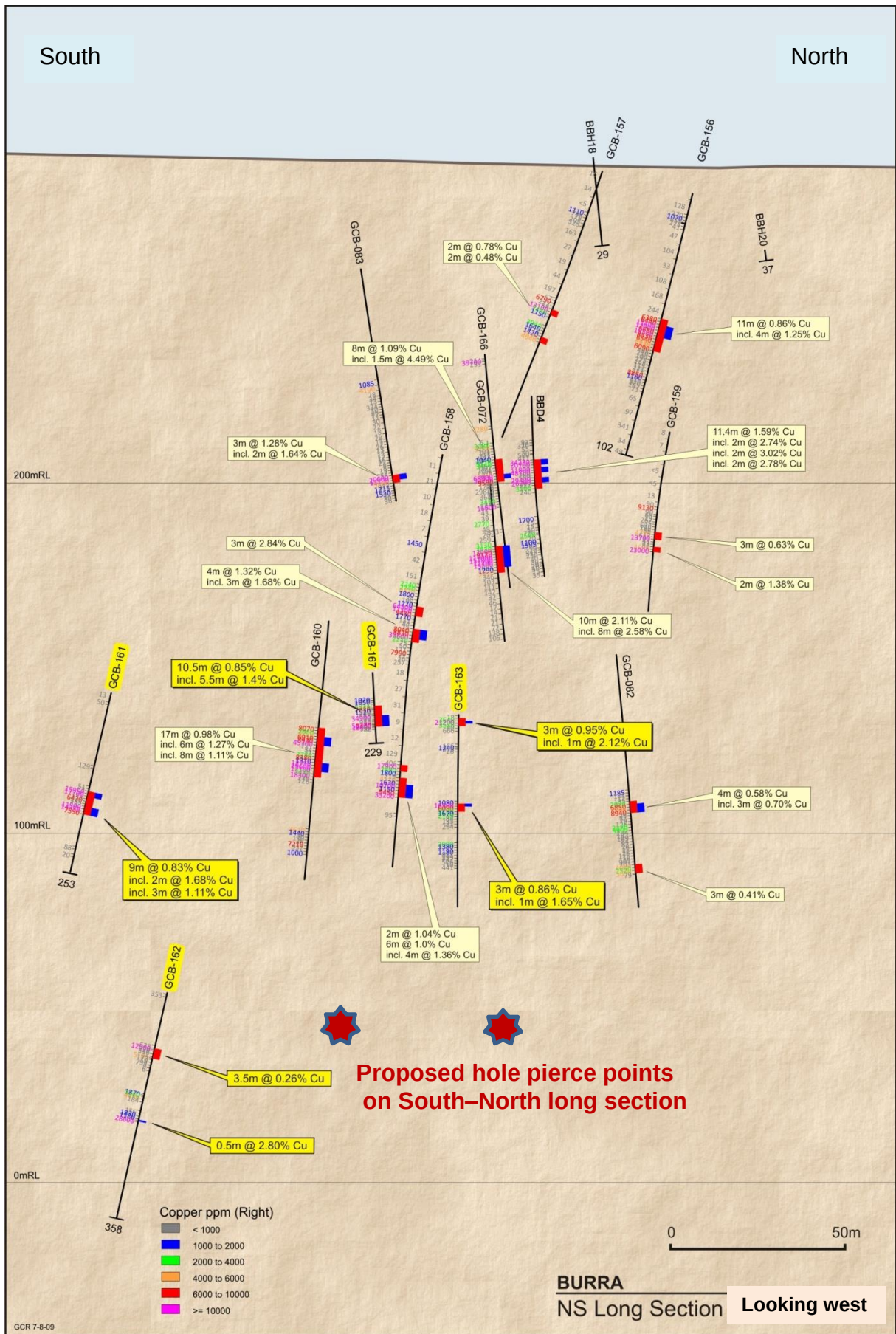
Burra Copper Mine Prospect: North-South Longitudinal Section
