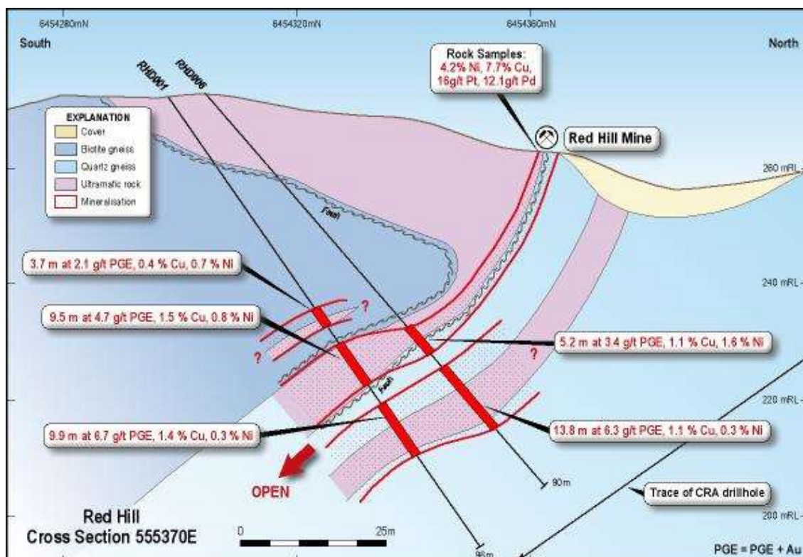
Figure 2. Cross Section along Line 555,370 mE.
