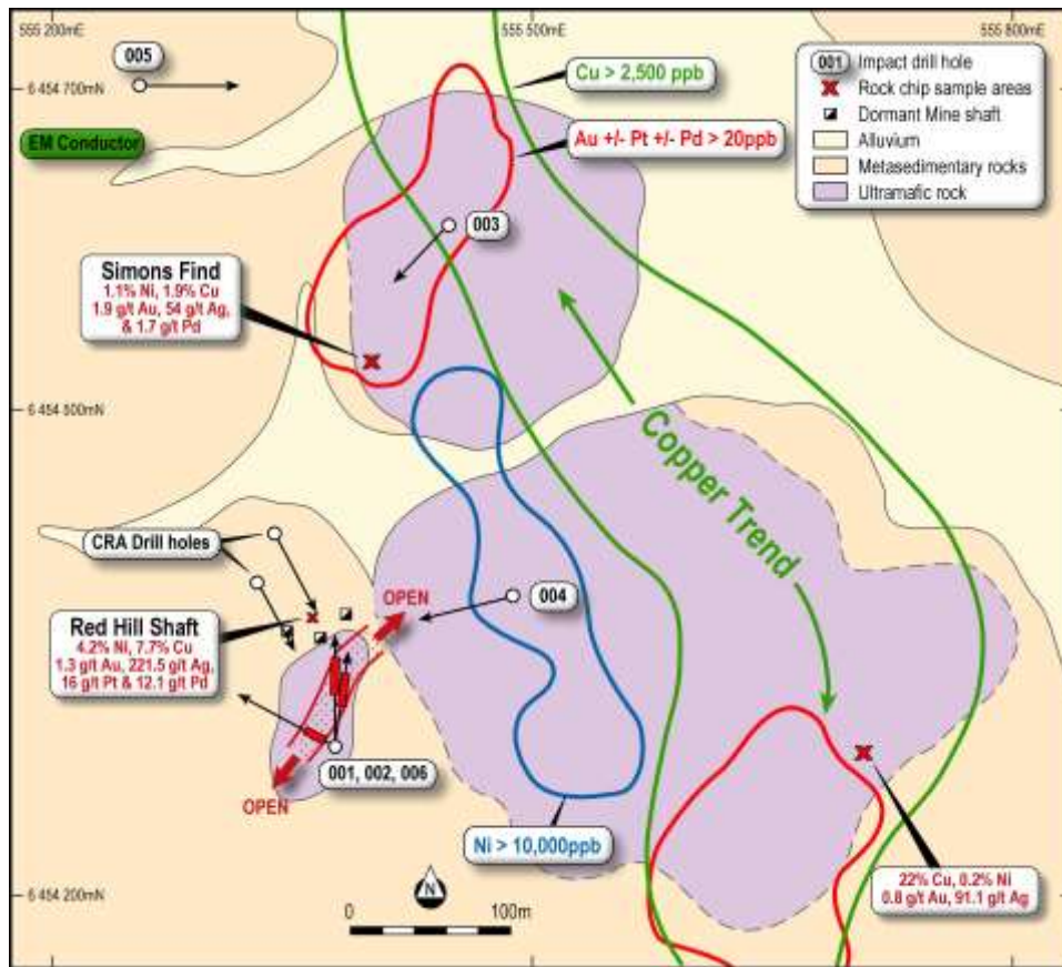
Figure 1. Geology, location of drill holes and mineralisation at the Red Hill Prospect.
