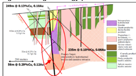
Figure 6: Section CYC12 & 13
