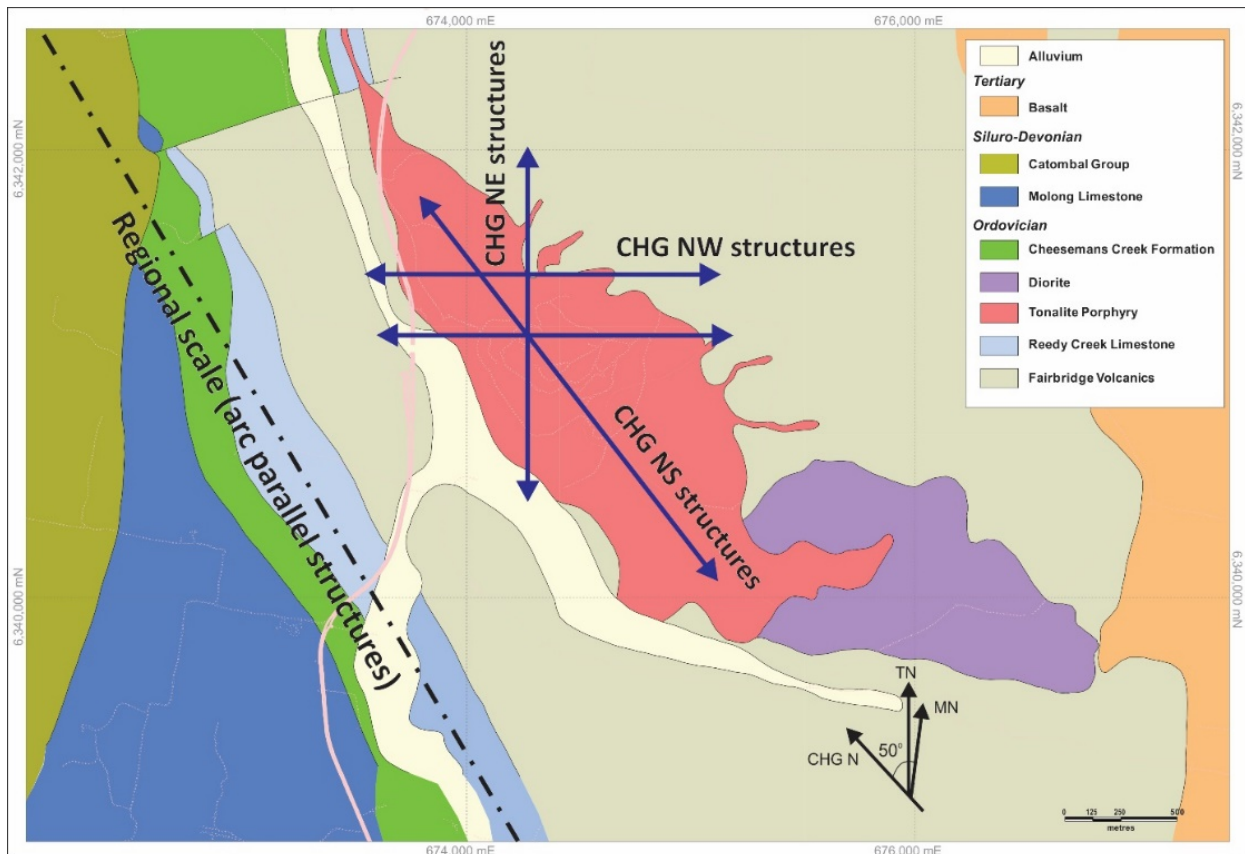
Figure 3: Copper Hill: Local Geology Map showing identified key structural orientations [Note: All structural directions in the text refer to local grid directions. Inset above shows relationship of the Copper Hill Local Grid North orientation which is rotated 50 degrees west of regional map north]
