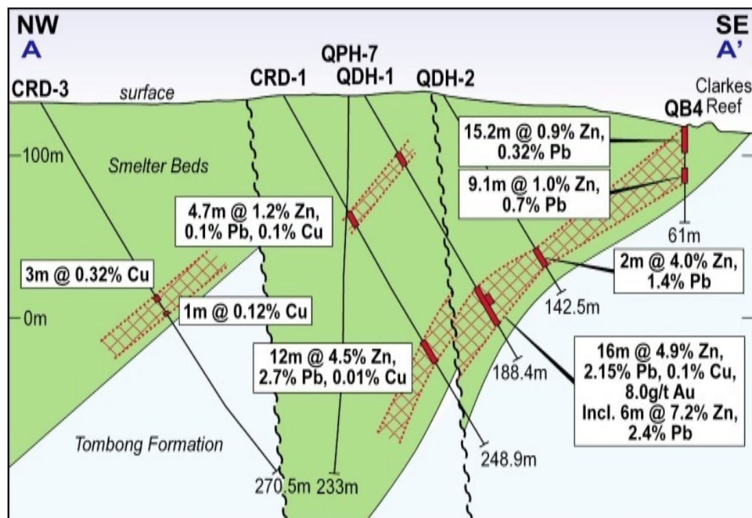
Figure 9 Typical Section: historical drilling at Clarke's Reef, southeast Quidong Basin
