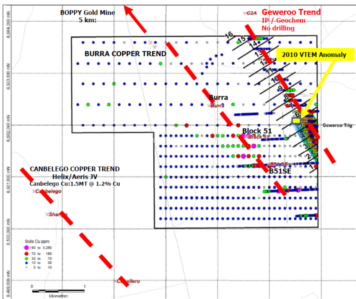
Figure 7: Burra EL7389 EM Lines on Geweroo Trend Targeting historical IP and 2010 VTEM anomaly
