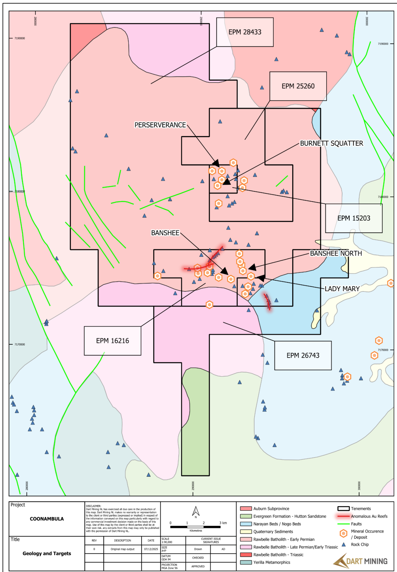
Figure 9: Coonambula geology and key prospects.
