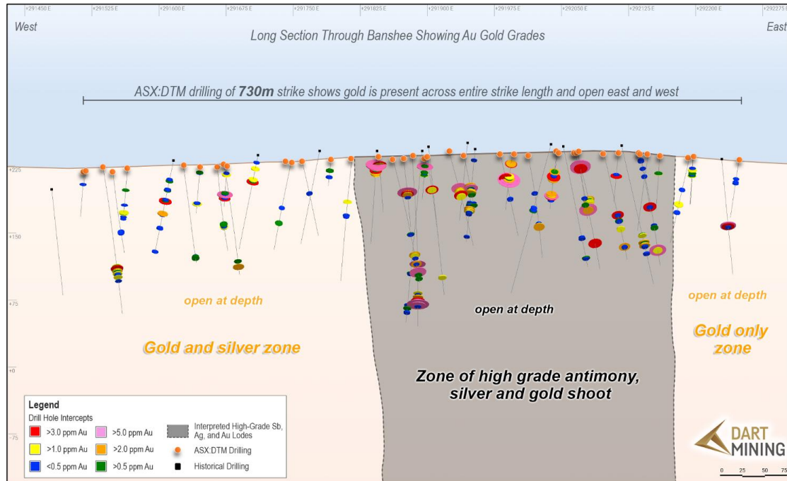
Long section through the drilling showing gold grades intercepted to date and interpretation of high-grade antimony and silver zones.
