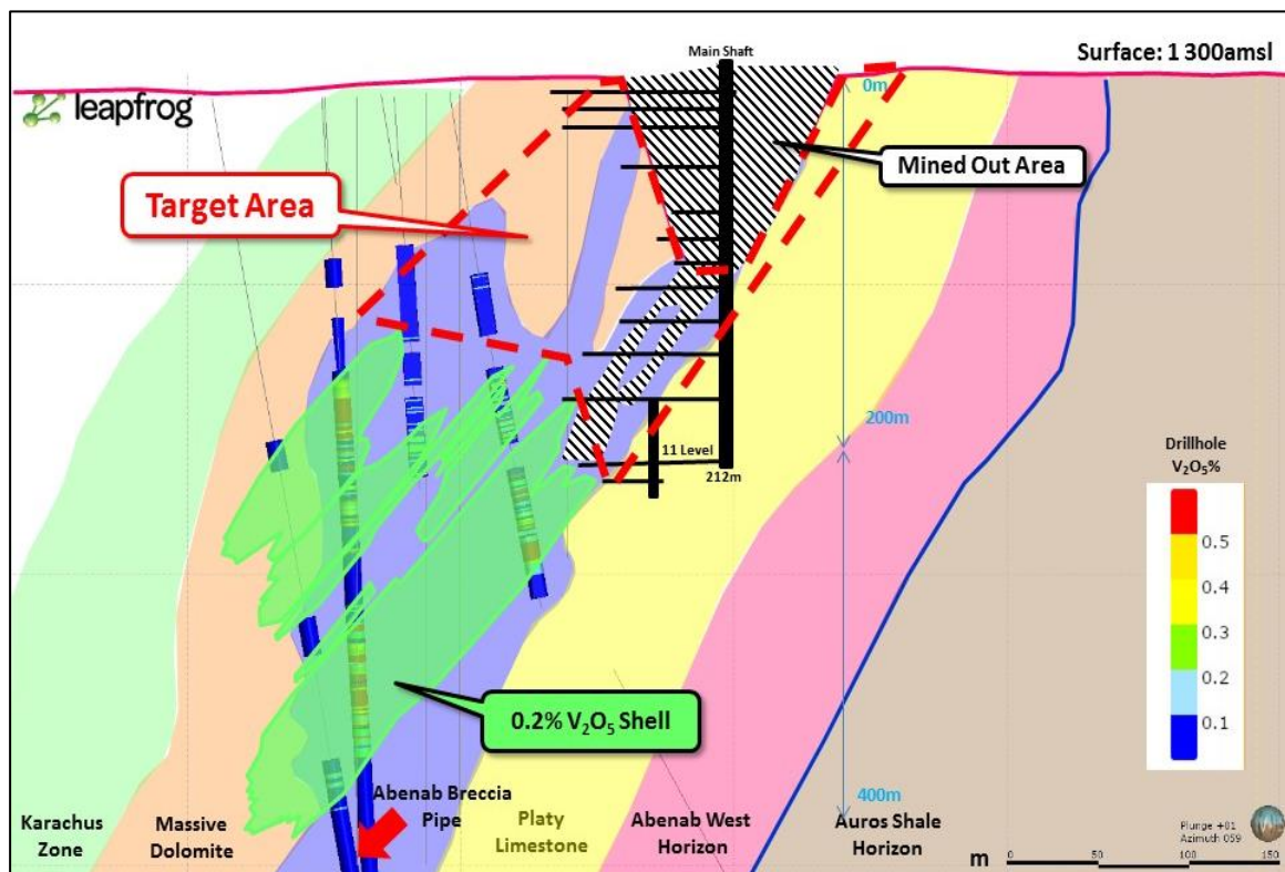
Figure 1: Cross section of Abenab mine showing the resource boundary at a 0.2% V_2O_5 cut off. Priority targets for resource extension drilling (red) include areas peripheral to the pit shell and extending down to the upper boundary of the resource.
