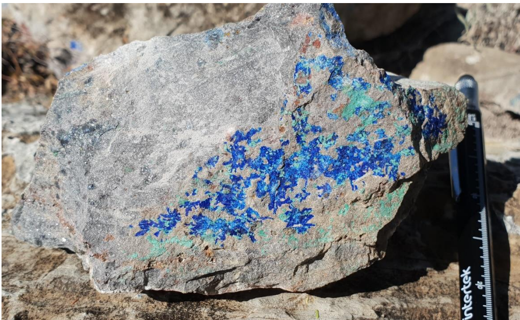
Photo 2: Copper mineralisation (azurite and malachite) above the Khusib Springs high-grade Cu-Ag deposit
