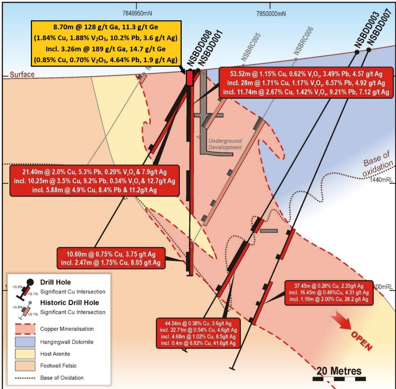
Figure 2: Nosib cross section through NSBDD008 showing at surface significant germanium and gallium intersection
