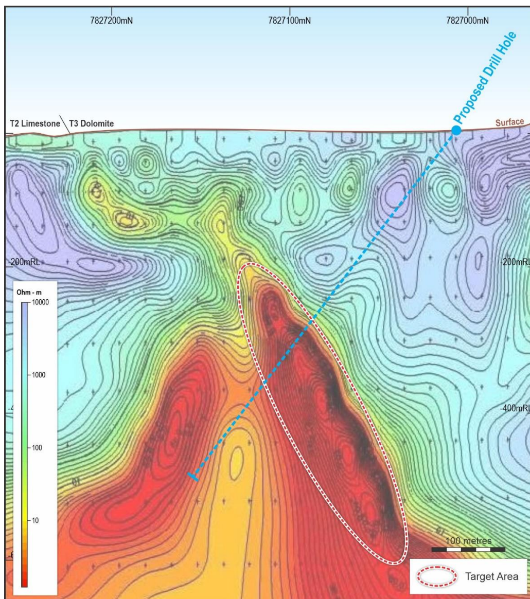
Figure 3: Major low-resistivity anomaly inversion model section 1600mE, with planned drilling.
