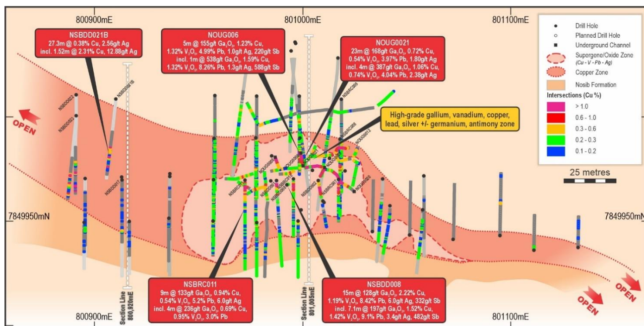
Figure 2: Nosib drilling, high-grade gallium (Cu, Pb, V, Ag, Ga +/- Ge, Sb) intersections & new drilling extending west
